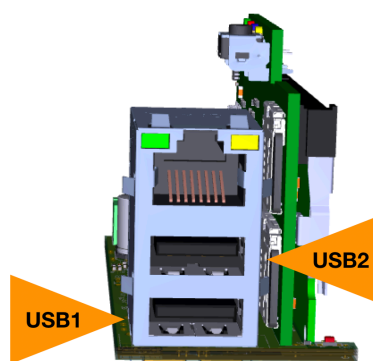
USB PORTS
