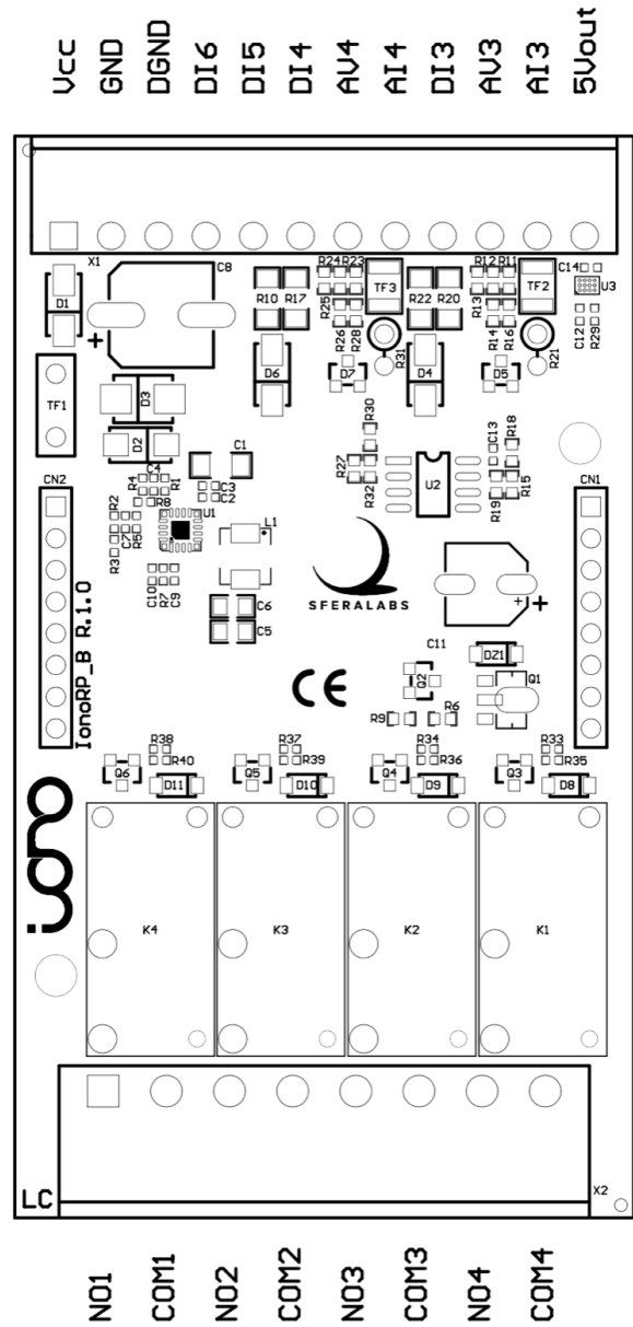
BOARD LAYOUT
