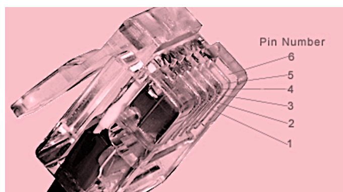
EXP INTERFACE PLUG PINS
