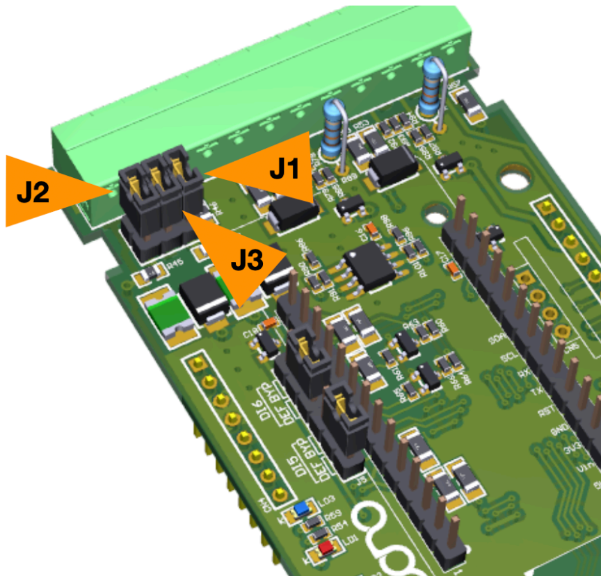
RS-485 JUMPERS POSITION
