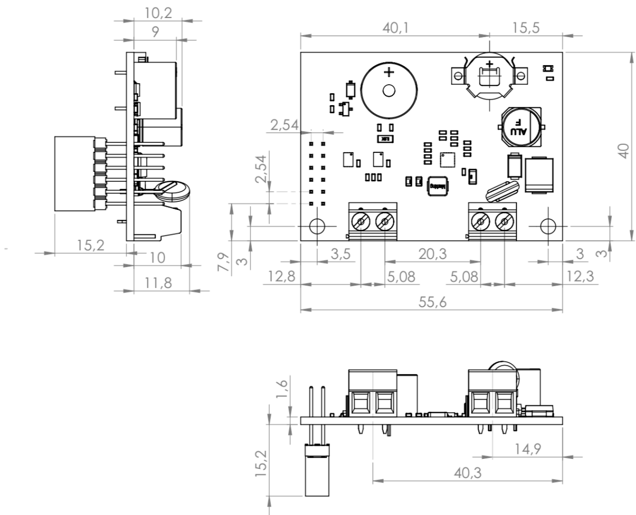
DIMENSIONS (mm)
