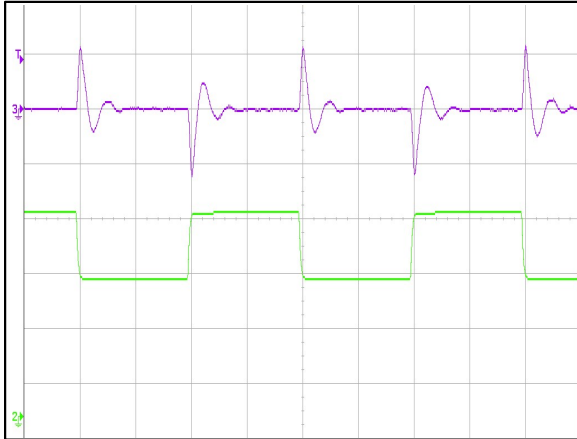
Figure 7: ADQ600B-48S12B Transient Response (2mS/div) 50%~75%~50% load change, 0.1A/uS slew rate, Vin = 48Vdc Ch 2: Io (10A/div) Ch 4: Vo (200mV/div)
