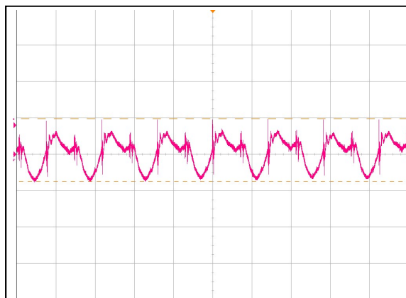
Figure 2: ADH700-48S50-6LS Ripple and Noise Measurement Ch1 : Vo (5uS/div, 50mV/div)
