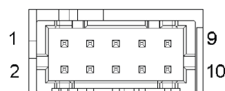
Figure 3: Connector CN1
