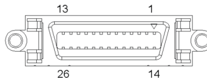
Figure 5: Connector CN3
