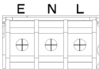
Figure 6: Input connector
