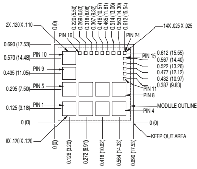
Recommended System Board Footprint
