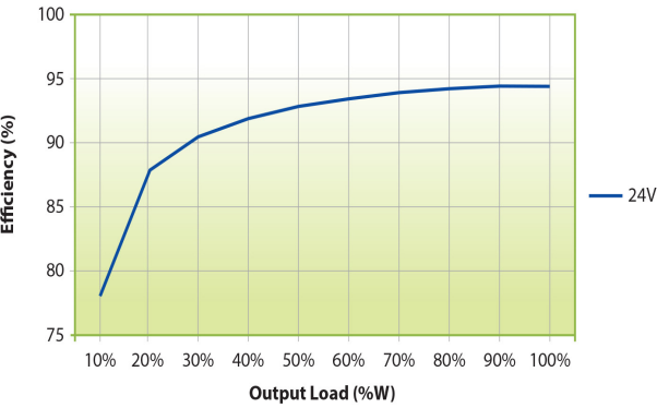
24V Model Efficiency Curve
