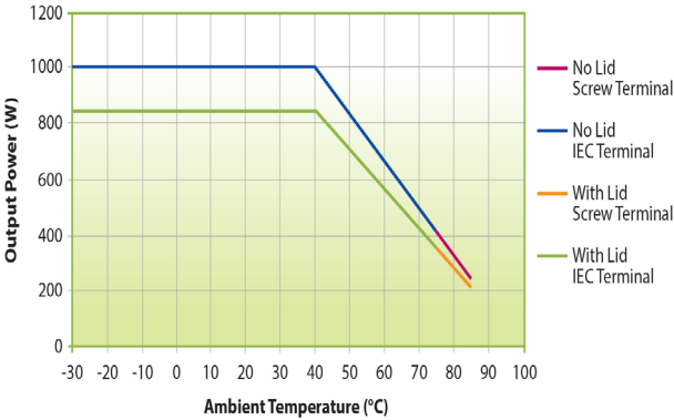
CS10 Temperature Derating Curve
