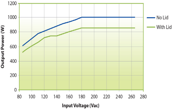
CS10 Input Voltage Typical Derating Curves
