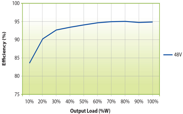
48V Model Efficiency Curve
