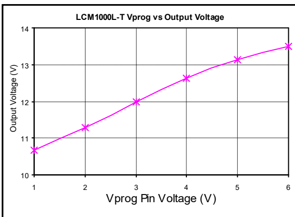
Figure 12: LCM1000L-T Output Voltage Adjustment by Vprog @ 25 °C
