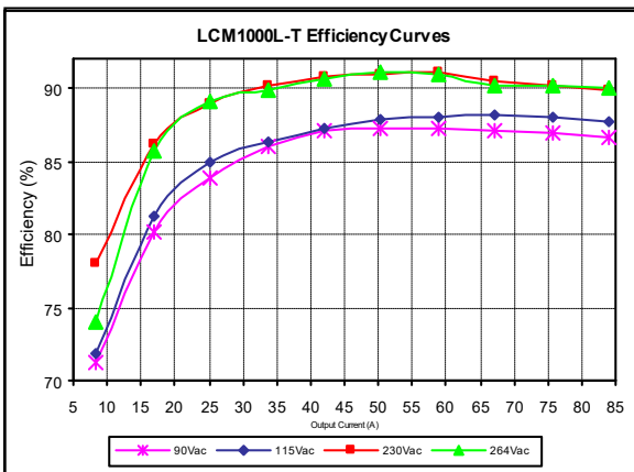
Figure 10: LCM1000L-T Efficiency Curves @ 25 °C
