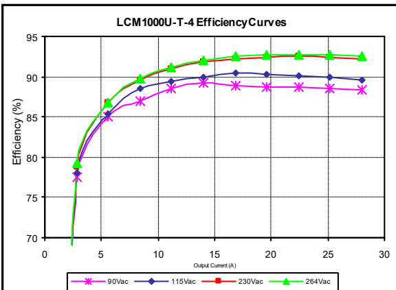
Figure 43: LCM1000U-T-4 Efficiency Curves @ 25 °C
