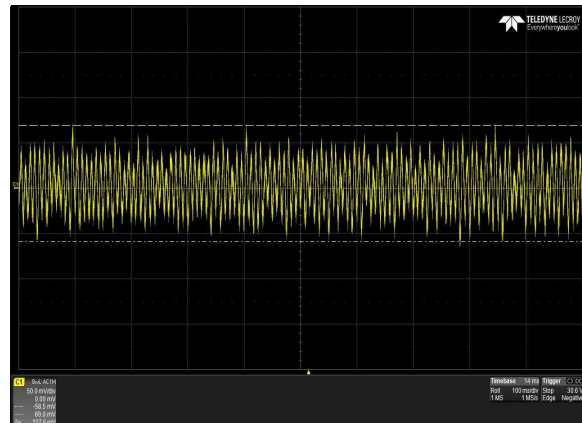
Figure 44: LCM1000U-T-4 Ripple and Noise Measurement – V_{IN} = 90\text{Vac} Full Load: I_O = 41.7\text{A} (36V)
