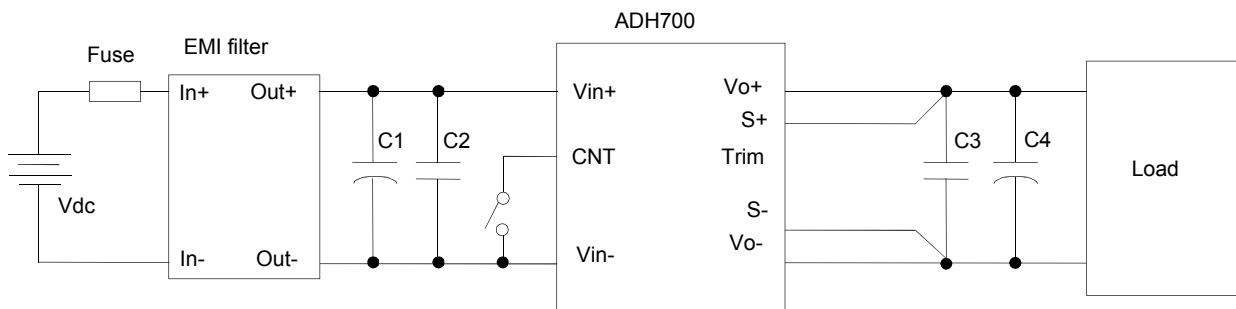
Figure 15: Typical application
