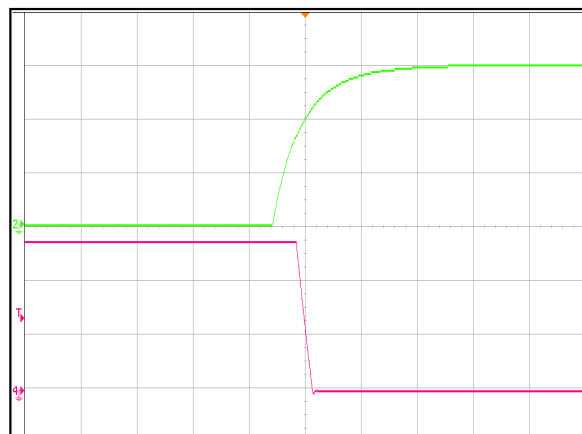
Figure 6: ADH700-48S28-6LS Output voltage shutdown by remote OFF Ch 2: Remote ON (2mS/div) (2V/div) Ch 4: Vo (10V/div)
