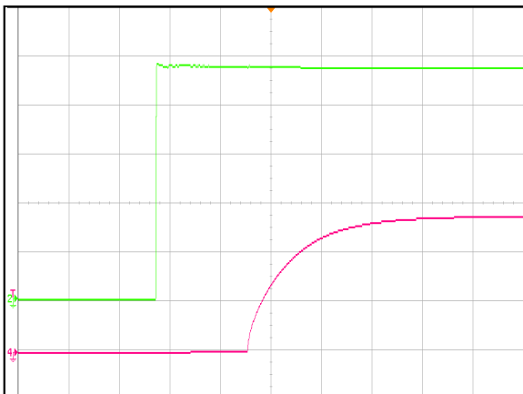
Figure 3: ADH700-48S28-6LS Output voltage startup by power on Ch 2: Vin (100mS/div) (10V/div) Ch 4: Vo (20V/div)
