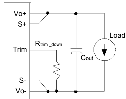
Figure 18: Trim down
