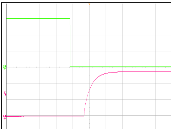
Figure 5: ADH700-48S28-6LS Output voltage startup by remote ON Ch 2: Remote ON (200mS/div) (2V/div) Ch 4: Vo (10V/div)
