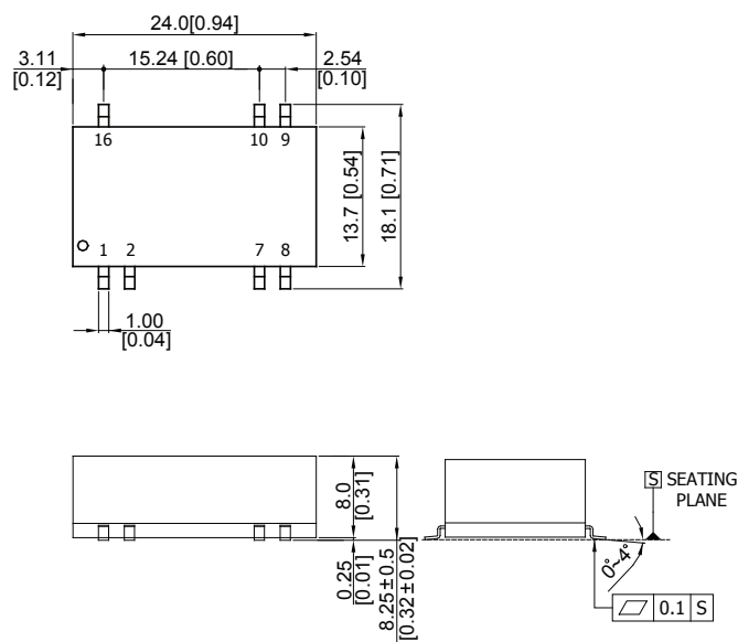
ATAxxxS-L (SMD)
