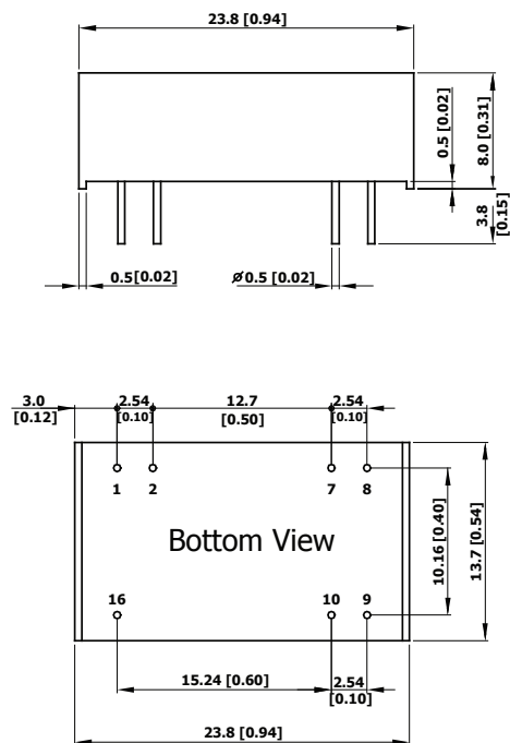
ATAxxx-L (DIP)
