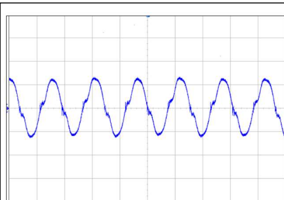
Figure 2: AVO120-48S12 Ripple and Noise Measurement
