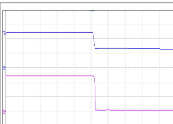
Figure 4: AVO120-48S12 Output Shutdown by Power Off (10ms/div)
