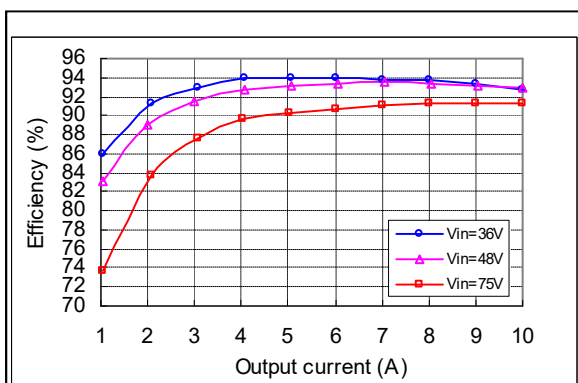
Figure 9: AVO120-48S12 Typical Efficiency V_{in} = 36-75Vdc , T_a=25^{\circ}C , V_o=12V , Air velocity=300LFM
