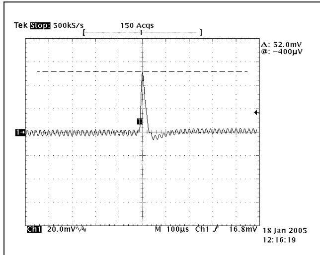
Figure 9. Transient Response at T_A = 25^\circ\text{C} , 12V OUT Deviation (Hi-Lo).
