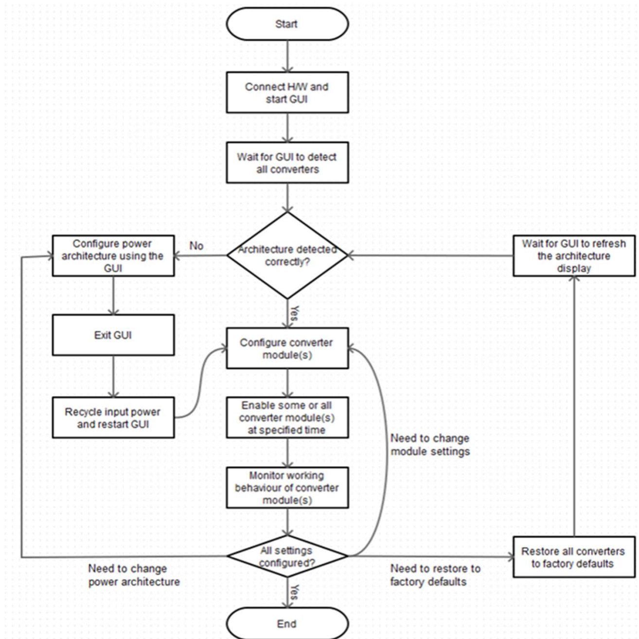
Figure 5. Programming Sequence
