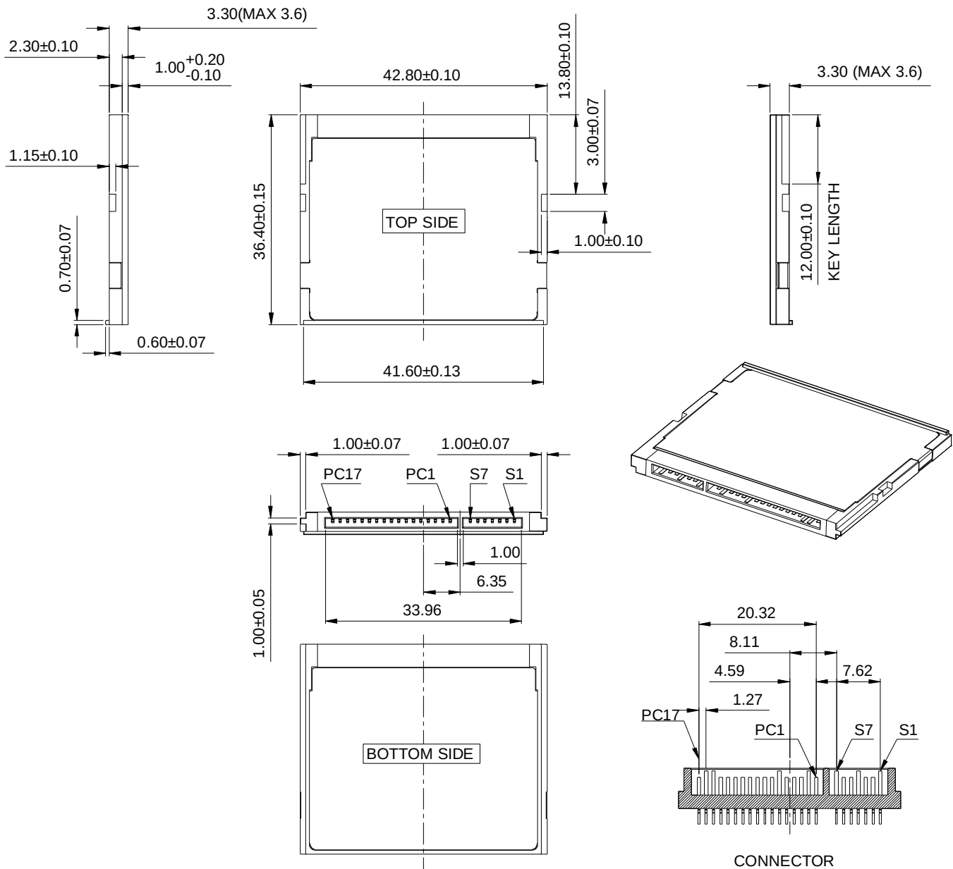
Figure 2: Mechanical Dimensions
