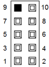
Socket Pinout
