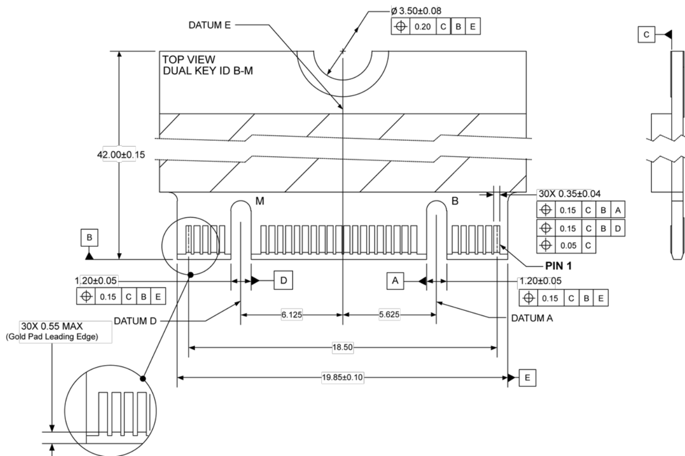
Figure 2: Connector Details
