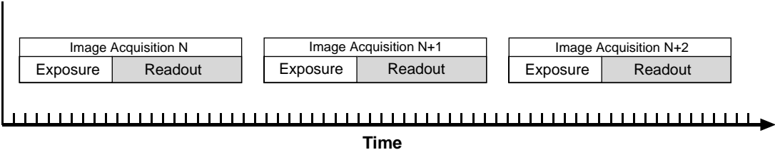
Fig. 59: Non-overlapped Exposure
