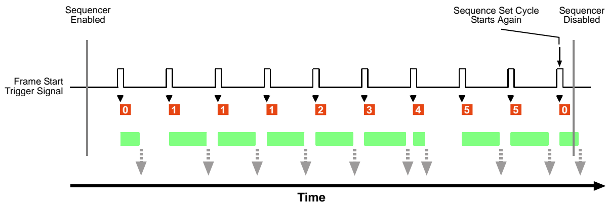
Fig. 73: Sequencer in Auto Sequence Advance Mode
