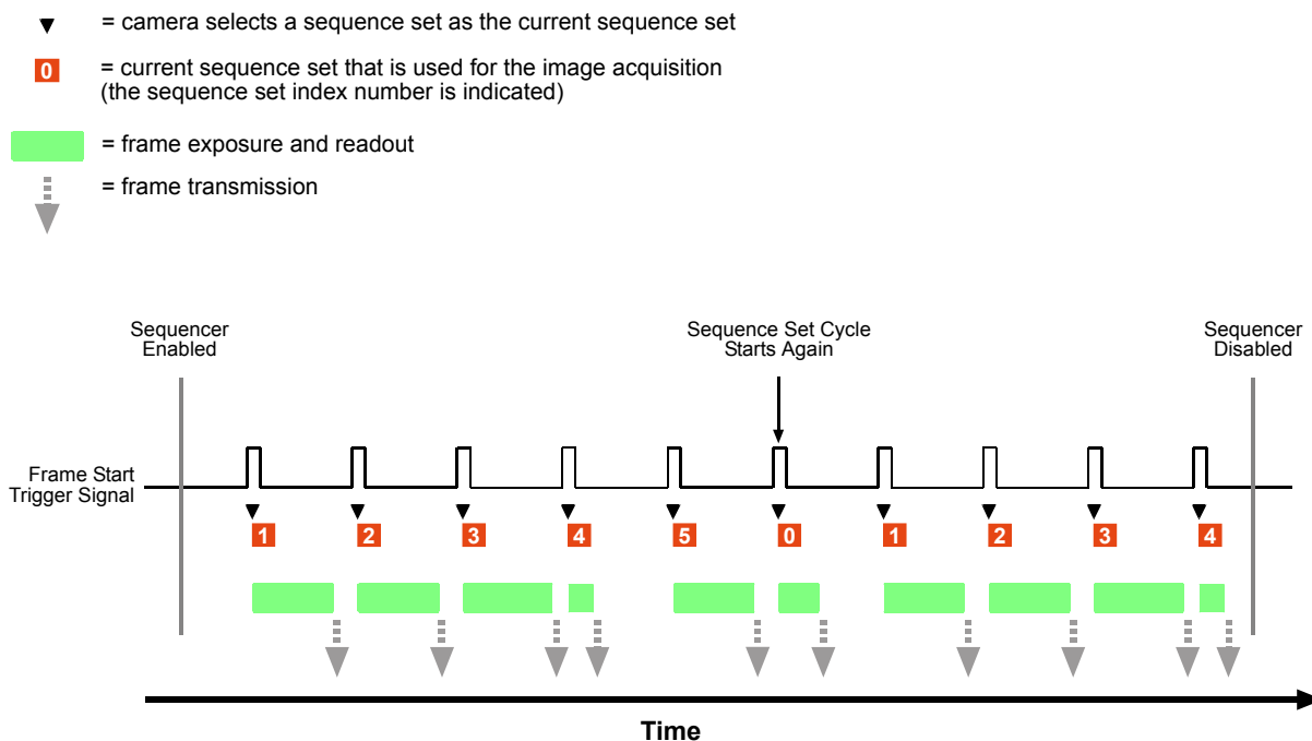
Fig. 59: Sequencer in Controlled Sequence Advance Mode with Always Active as the Sequence Control Source
