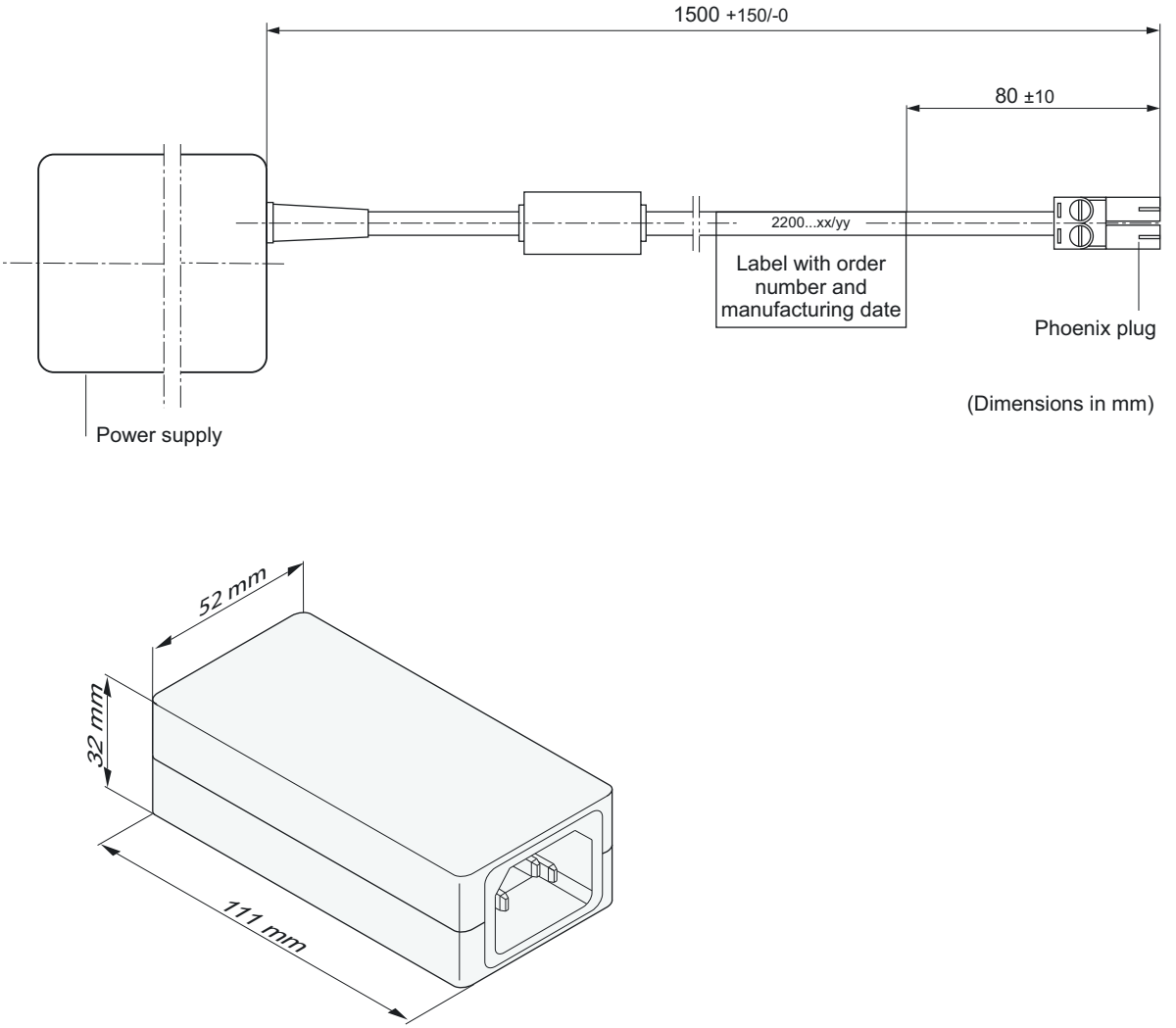
Fig. 1: Power Supply Overview
