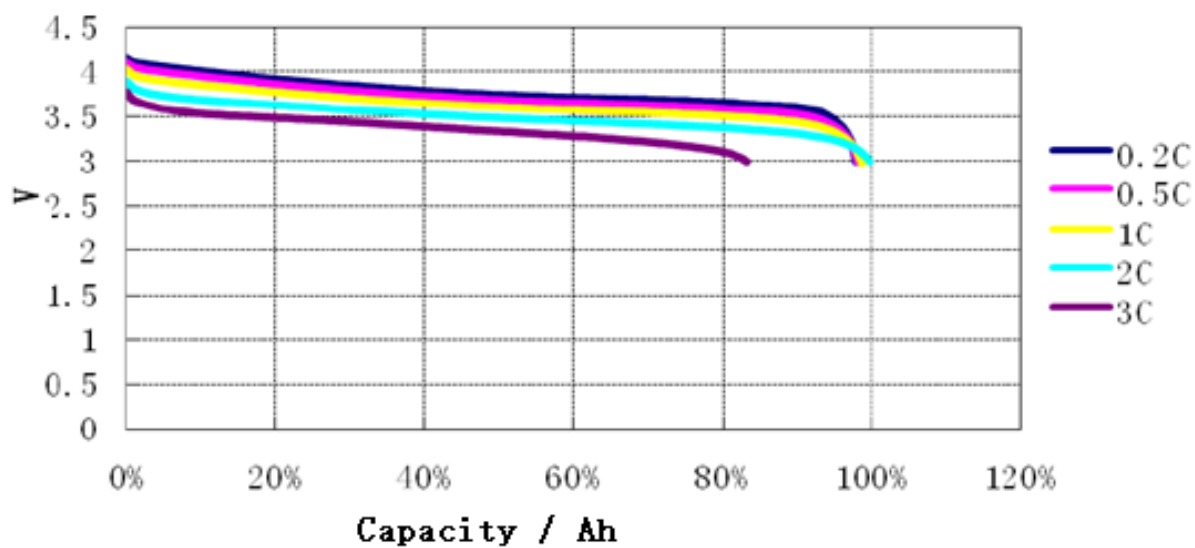
Figure 3: 1000mAh Battery Discharging Characteristics
