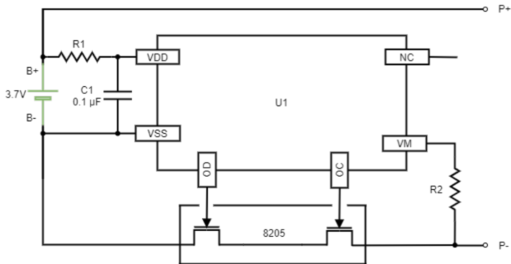
Figure 4: 1000mAh Battery Schematic
