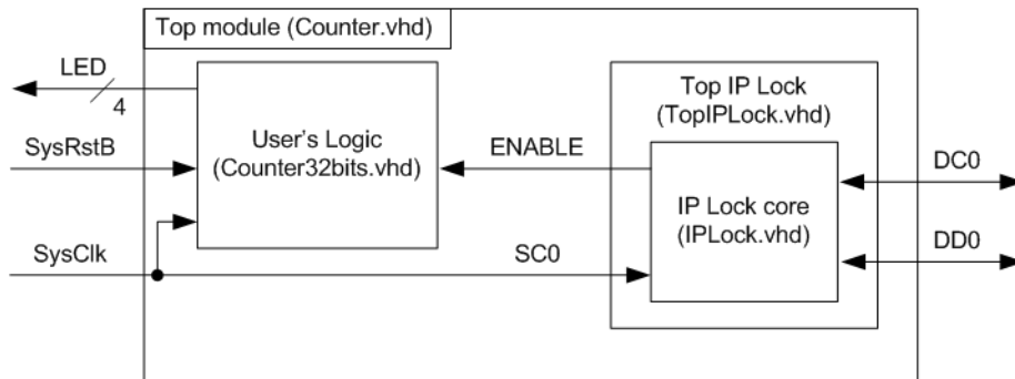
Figure 2-7 Example VHDL design block diagram
