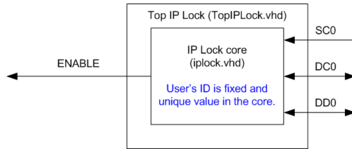
Figure 2-3 Top level of IP Lock
