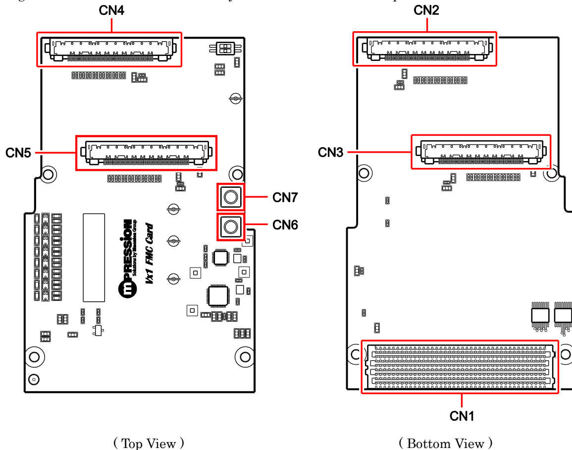
Figure 4-2 Connector Layout
