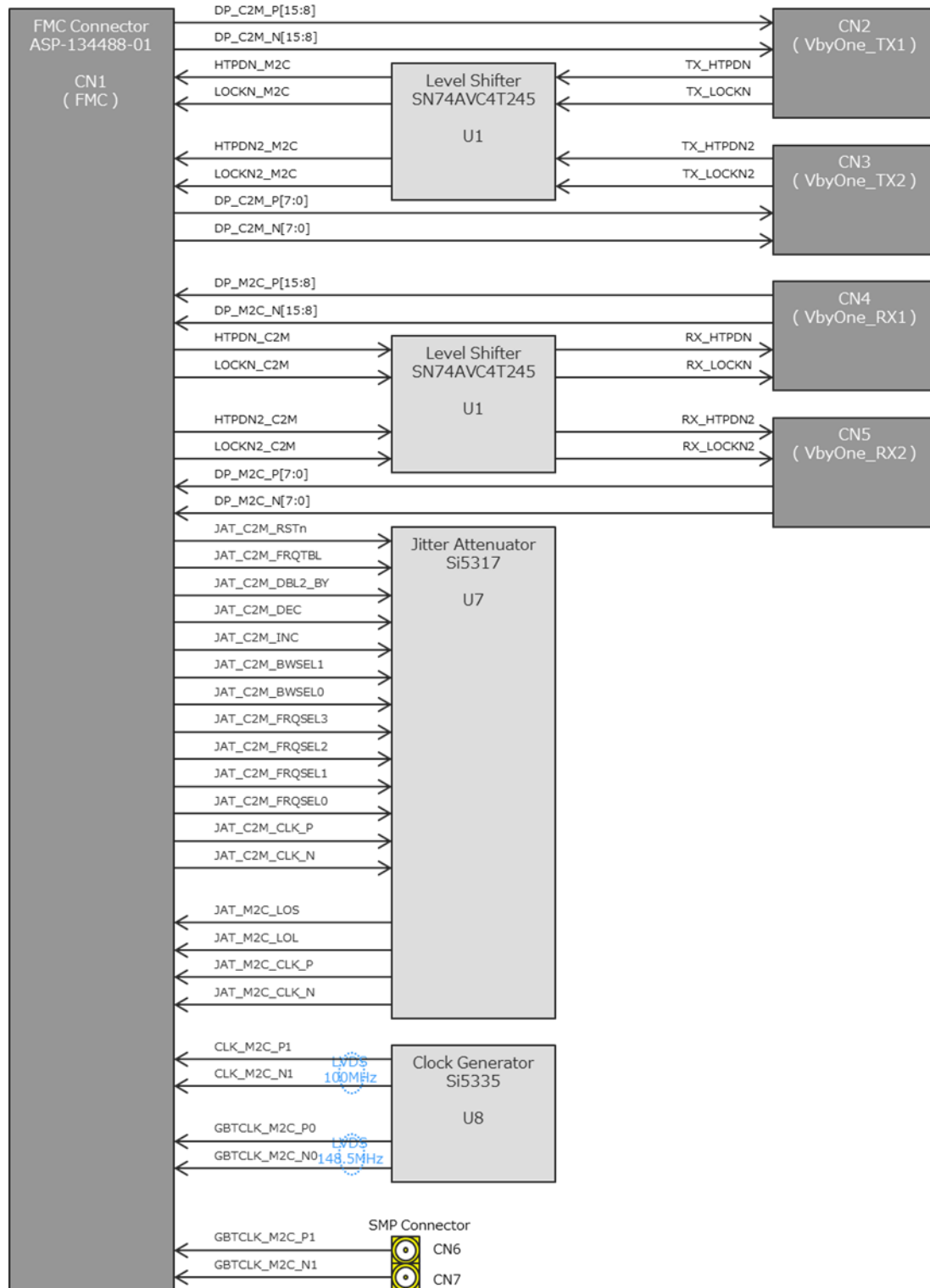
Figure 4-1 Block Diagram
