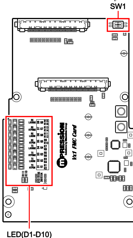
Figure 4-4 Switch and LED Layout
