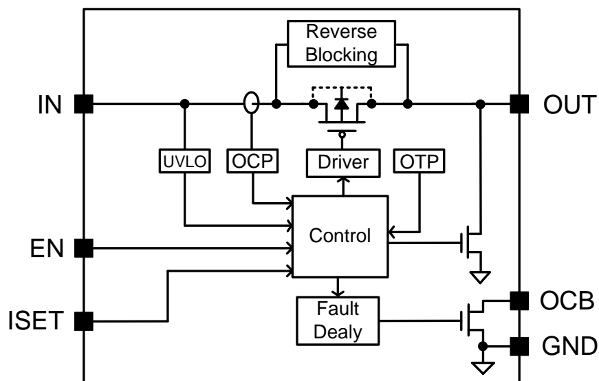
Figure 2. Block Diagram
