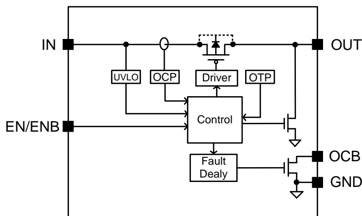
Figure 2. Block Diagram
