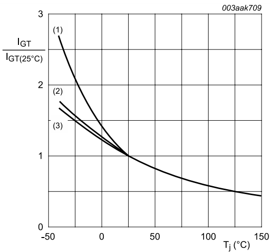
(1) T2- G- (2) T2+ G- (3) T2+ G+ Fig. 7. Normalized gate trigger current as a function of junction temperature
