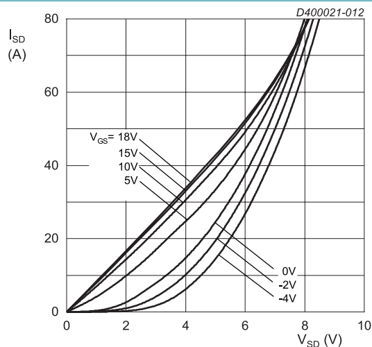
T_j = 175^\circ\text{C} ; t_p < 200\ \mu\text{s} Fig. 12. Body diode forward characteristics; typical values
