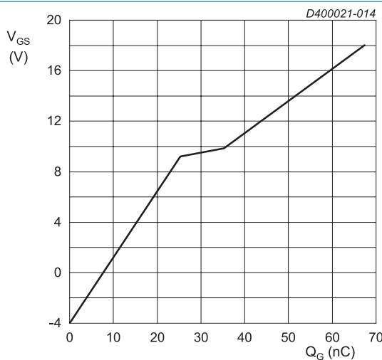
I_{DS} = 20\ \text{A} ; I_{GS} = 0.1\ \text{mA} ; V_{DS} = 800\ \text{V} ; T_j = 25^\circ\text{C} Fig. 14. Gate-source voltage as a function of gate charge; typical values
