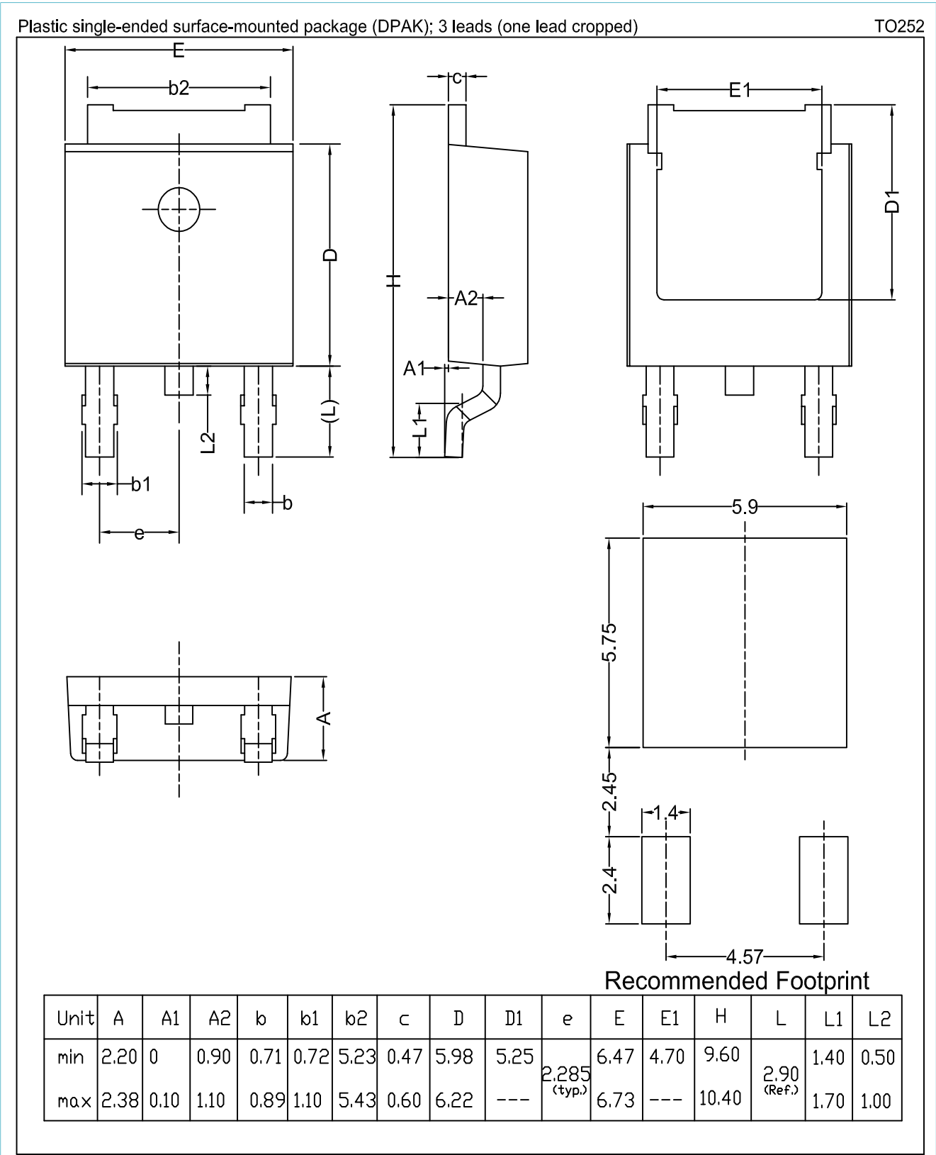
Fig. 8. Package outline DPAK (TO252NS) NXPSC10650D All information provided in this document is subject to legal disclaimers. © WeEn Semiconductors Co., Ltd. 2017. All rights reserved Product data sheet 4 January 2017 7 / 10
