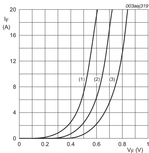
(1) T_j = 125\text{ }^\circ\text{C} ; typical values; (2) T_j = 125\text{ }^\circ\text{C} ; maximum values; (3) T_j = 25\text{ }^\circ\text{C} ; maximum values; V_O = 0.516\text{ V} ; R_S = 0.010\text{ }\Omega
