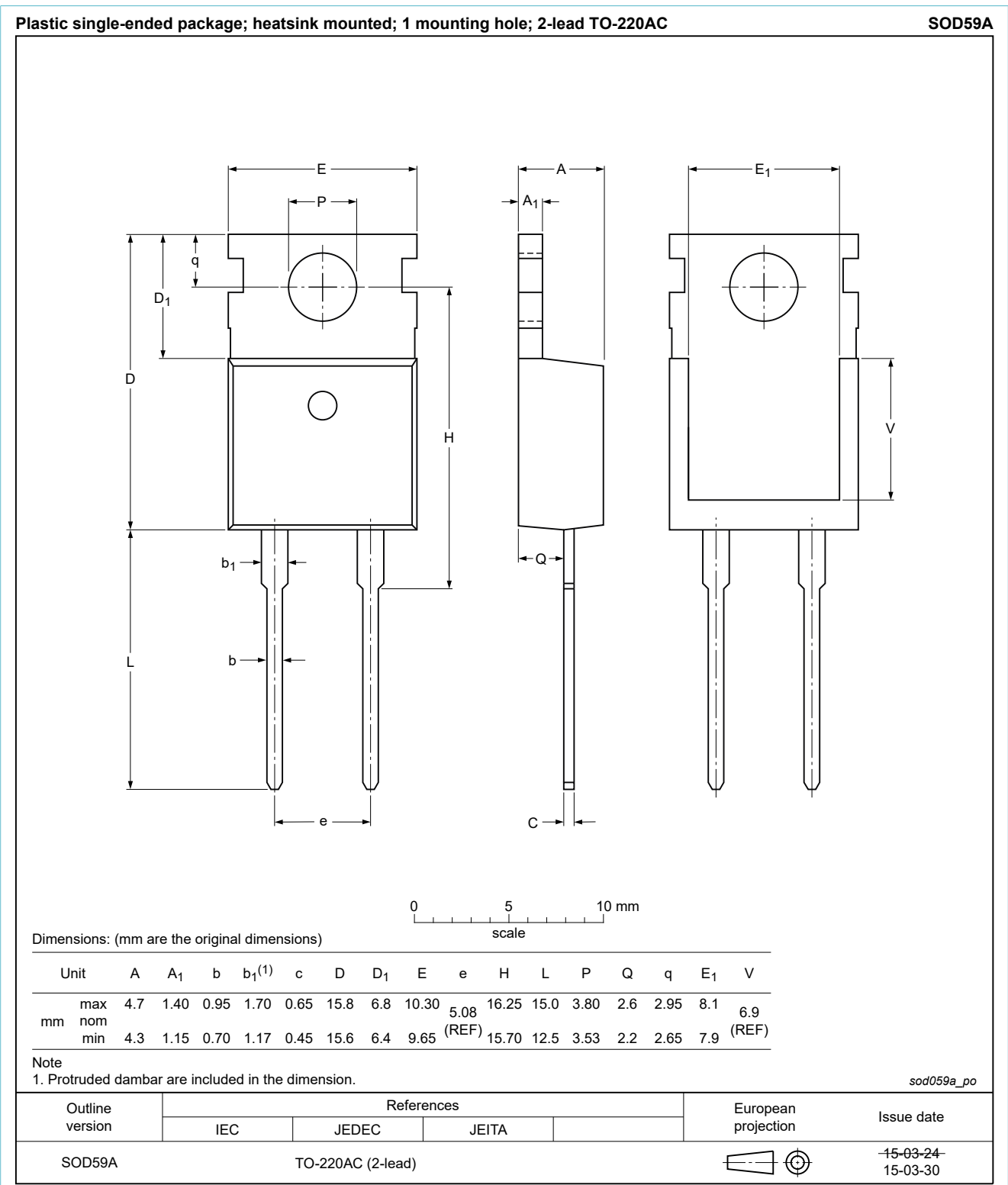
Fig. 7. Package outline TO-220AC (SOD59A)
