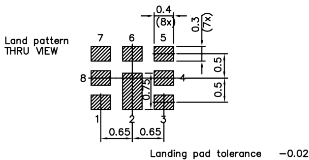
Figure 2: Drawing of package with package height A = 0.64 mm (max.). See Sec. Package information (p. 20).
