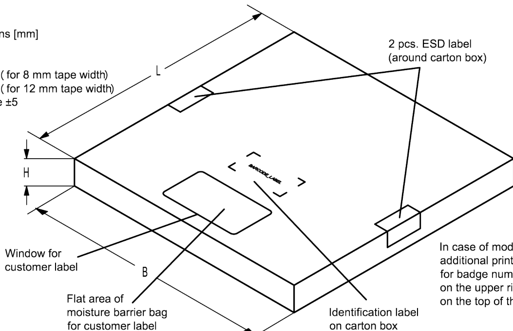
Figure 13: Drawing of folding box for reel with diameter of 330 mm.
