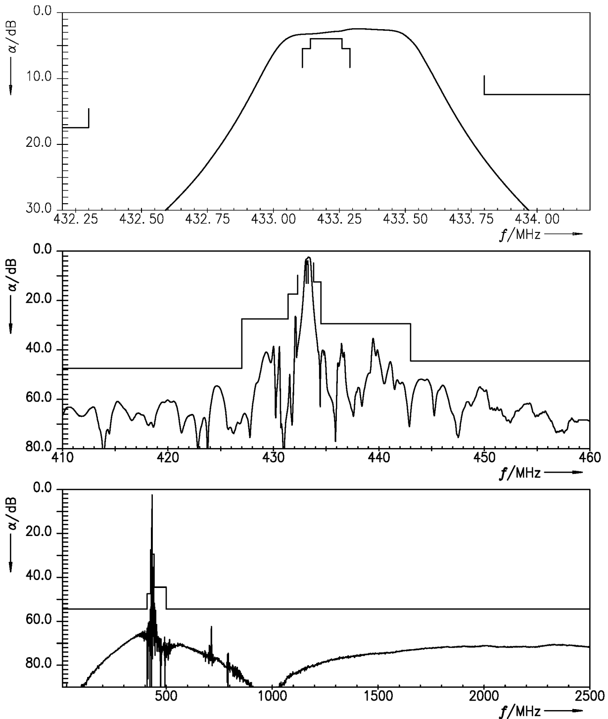
Figure 6: Attenuation Channel 3.
