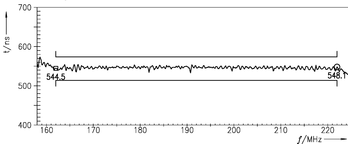
Figure 6: Group delay.
