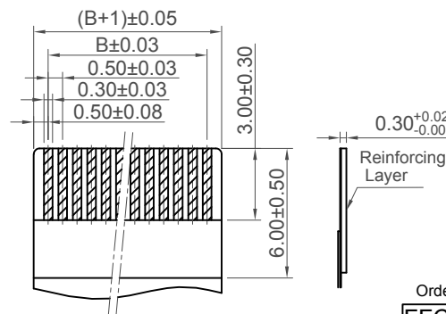
Recommended FFC/FPC Dimensions
