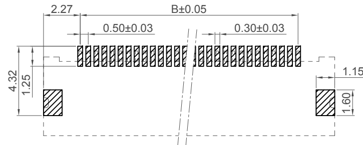
Recommended PCB Layout General Tolerance \pm 0.05
