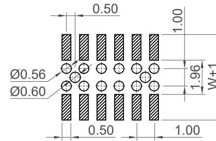
Recommended PCB Layout For Bottom Entry General Tolerance: \pm 0.05 Solder Area
