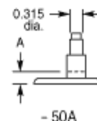
Momentary - For Auxiliary Push Button
