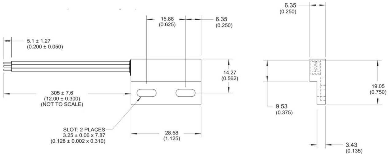
MAGNETIC ACTUATOR AS201901
