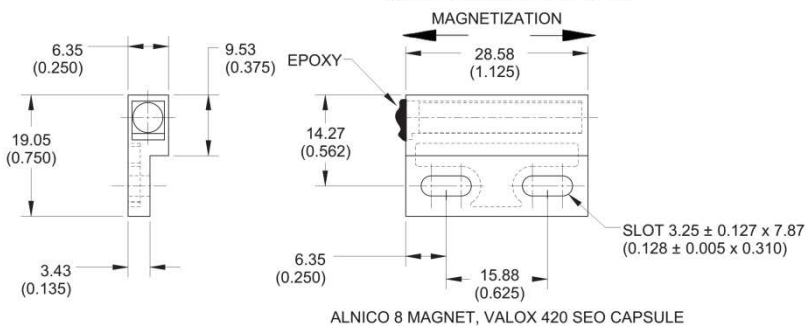
MAGNETIC ACTUATOR AS201901
