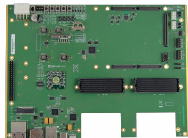
Zeus Carrier board 170mm x 233.35mm
