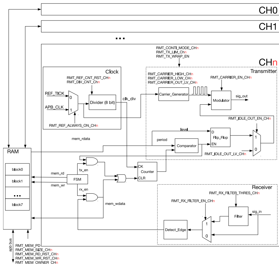
Figure 15-1. RMT Architecture
