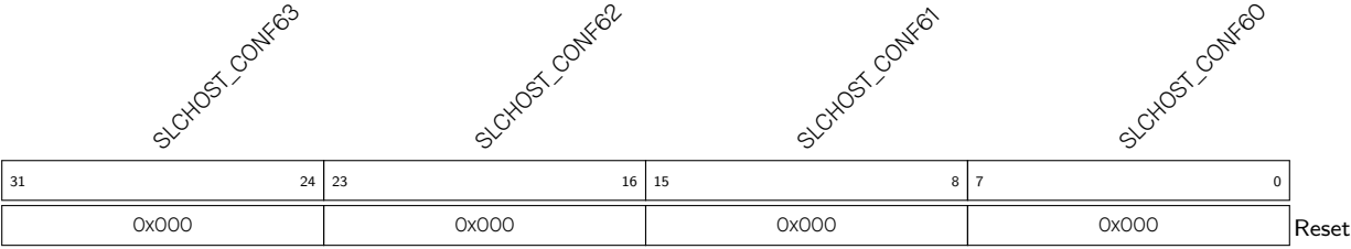
Register 8.31. SLCHOST_CONF_W15_REG (0xB8)
