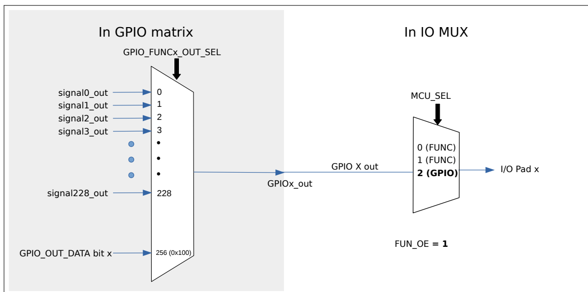
Figure 4-4. Output via GPIO Matrix
