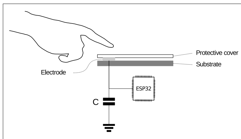
Figure 29-1. Touch Sensor
