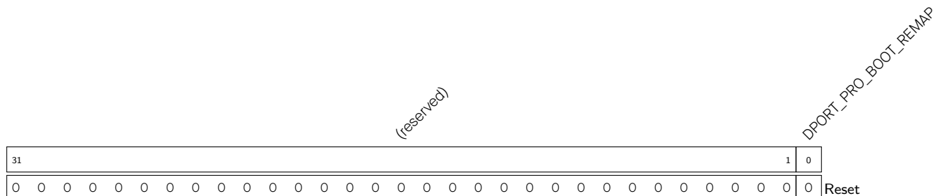
Register 5.1. DPORT_PRO_BOOT_REMAP_CTRL_REG (0x000)
