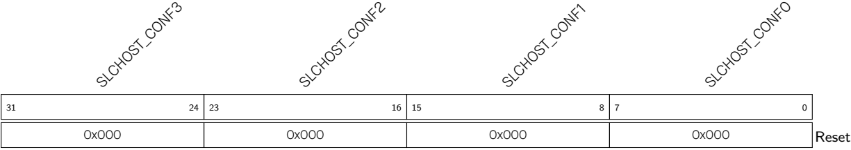
Register 8.18. SLCHOST_CONF_WO_REG (0x6C)
