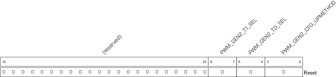
Register 16.47. PWM_GEN2_CFG0_REG (0x00b8)
