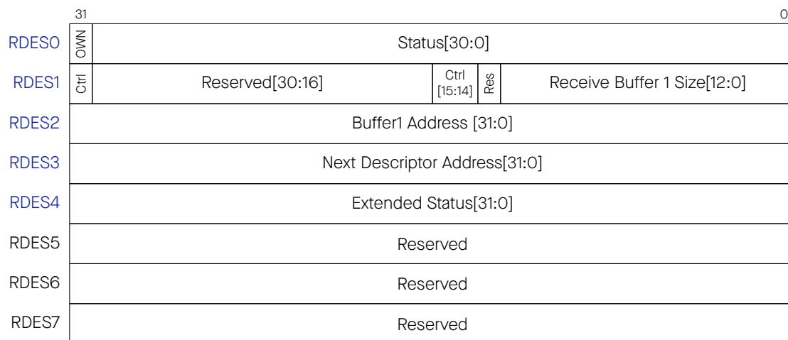
Figure 10-10. Receive Descriptor
