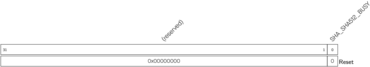
Register 23.17. SHA_SHA512_BUSY_REG (0x0BC)
