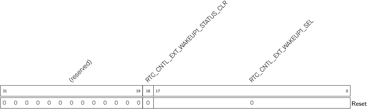
Register 31.37. RTC_CNTL_EXT_WAKEUP1_REG (0x00CC)
