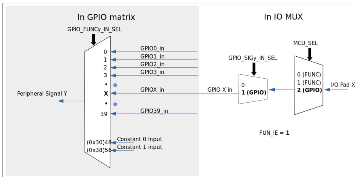
Figure 4-3. Peripheral Input via IO MUX, GPIO Matrix
