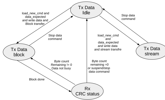
Figure 9-5. Data Transmit State Machine
