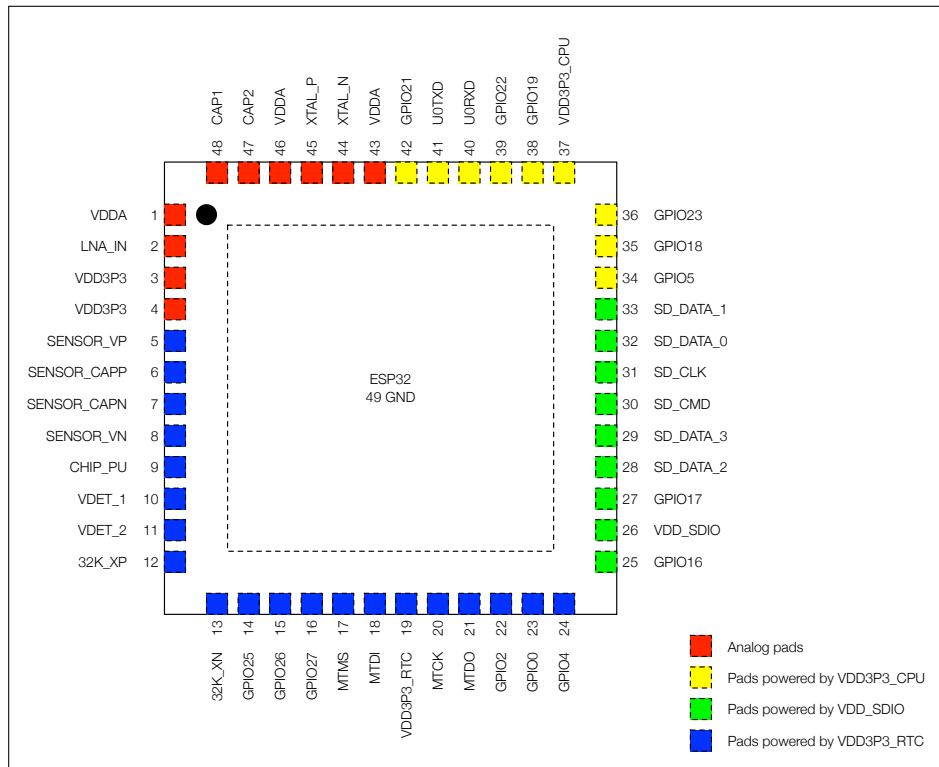
Figure 4-5. ESP32 I/O Pin Power Sources (QFN 6*6, Top View)
