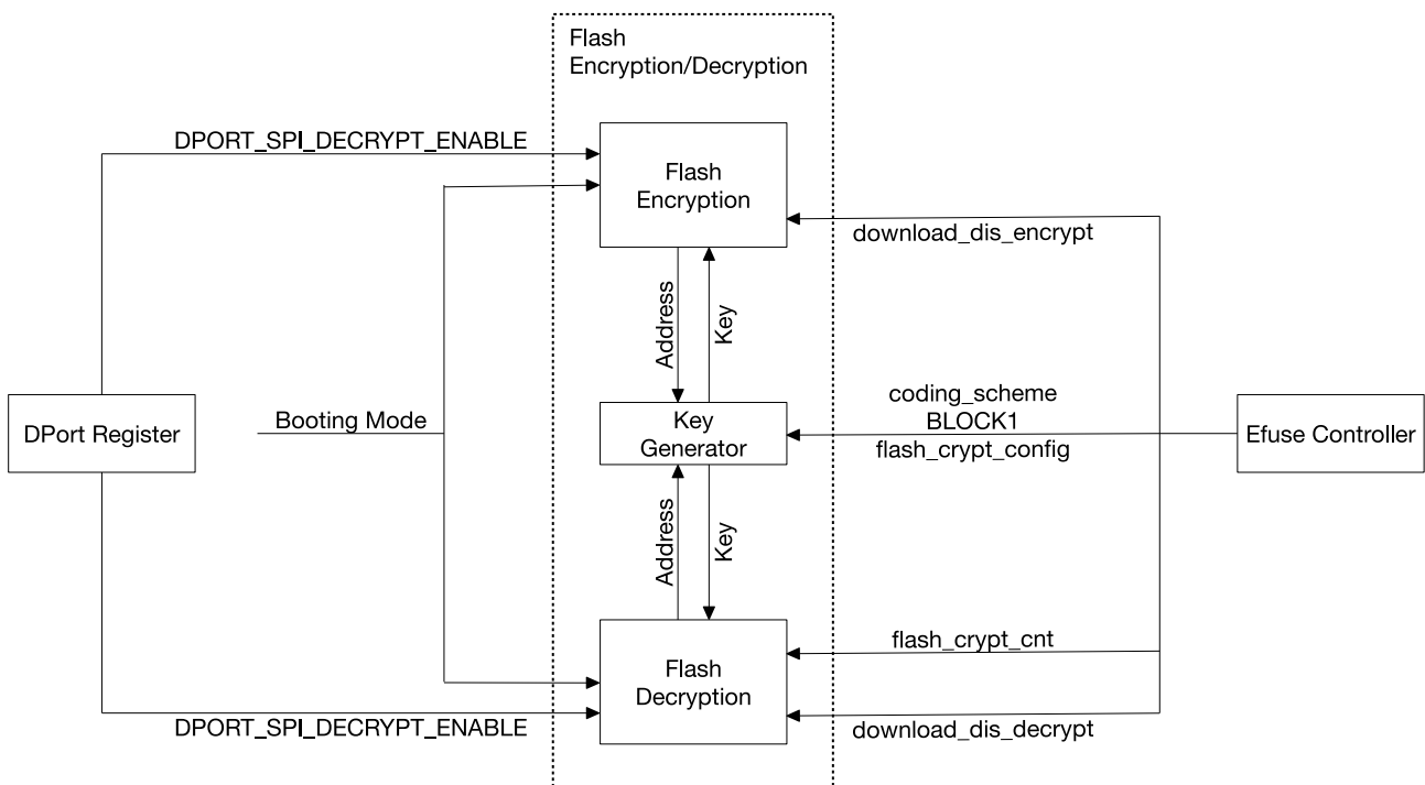
Figure 26-1. Flash Encryption/Decryption Module Architecture
