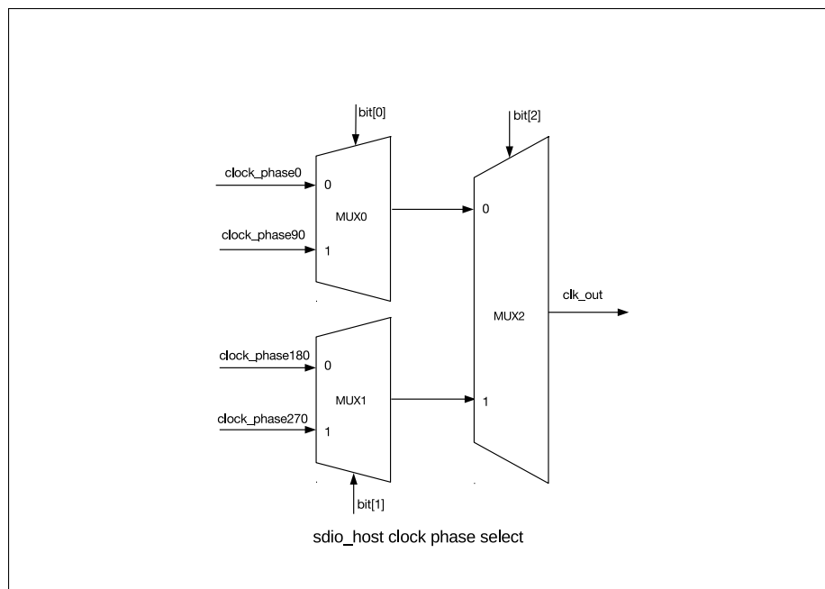
Figure 9-10. Clock Phase Selection
