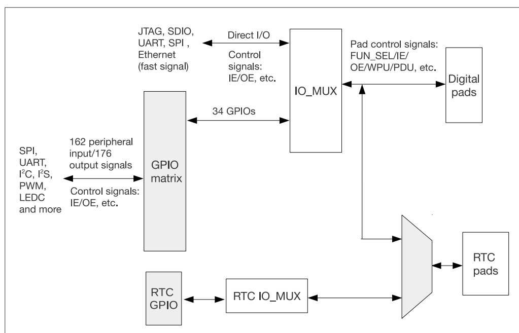
Figure 4-1. IO MUX, RTC IO MUX and GPIO Matrix Overview
