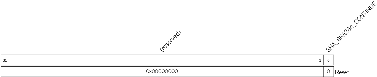
Register 23.11. SHA_SHA384_CONTINUE_REG (0x0A4)
