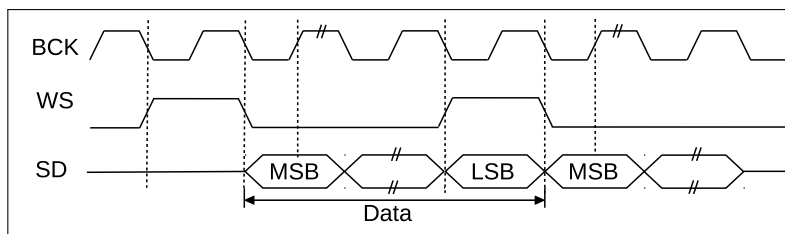
Figure 12-5. PCM Standard
