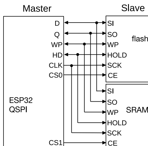
Figure 7-5. Parallel QSPI
