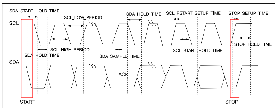
Figure 11-3. I2C Sequence Chart
