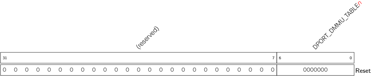
Register 5.193. DPORT_DMMU_TABLE n _REG ( n : 0-15) (0x544+4* n )
