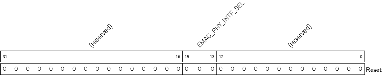
Register 10.47. EMAC_EX_PHYINF_CONF_REG (0x080C)
