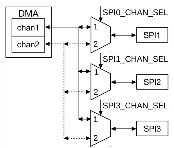
Figure 6-4. SPI DMA
