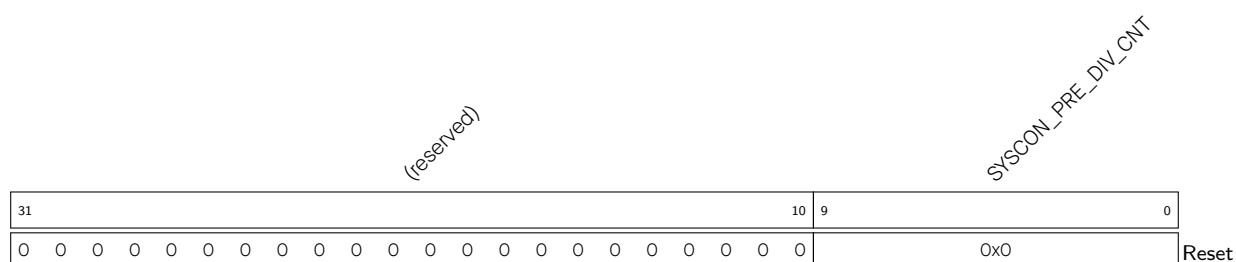
Register 3.1. SYSCON_SYSCLOCK_CONF_REG (0x0000)
