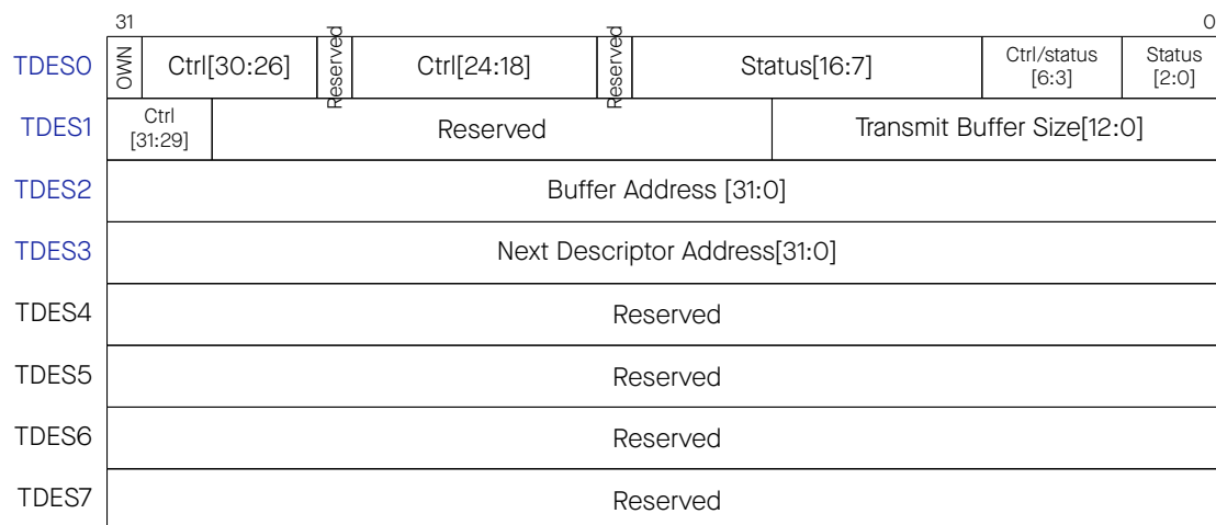
Figure 10-9. Transmit Descriptor
