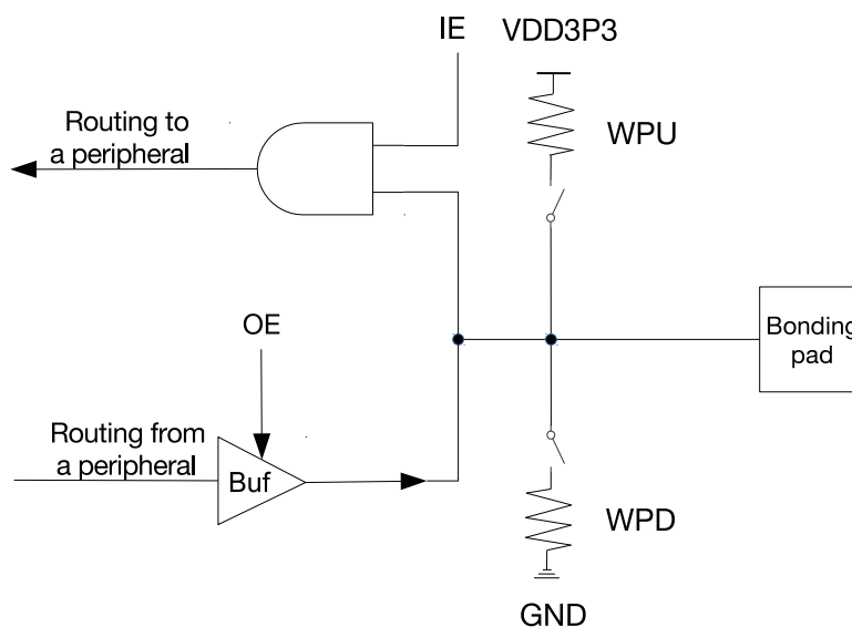
Figure 4-2. Internal Structure of a Pad
