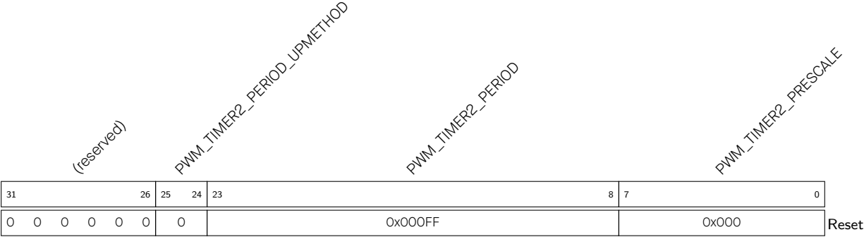
Register 16.10. PWM_TIMER2_CFG0_REG (0x0024)
