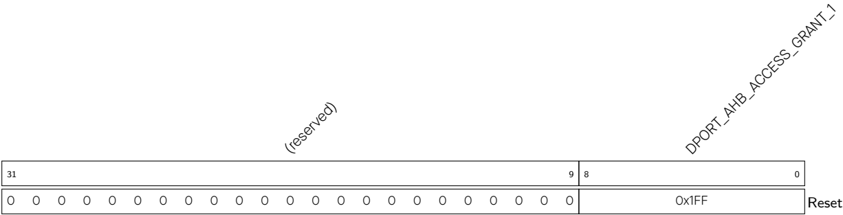
Register 5.18. DPORT_AHB_MPU_TABLE_1_REG (0x0B8)
