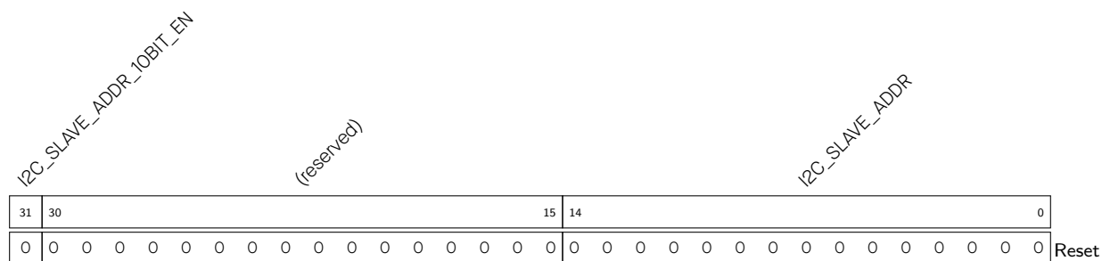
Register 11.5. I2C_SLAVE_ADDR_REG (0x0010)
