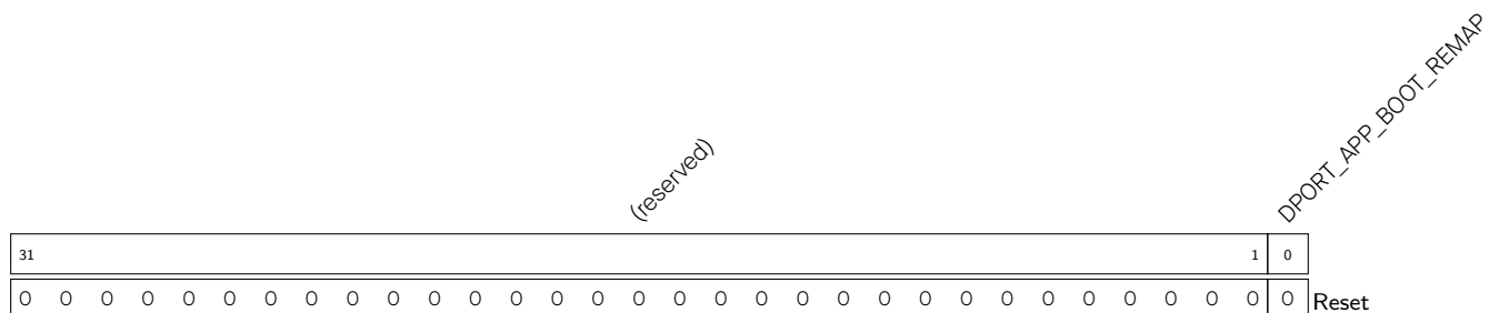
Register 5.2. DPORT_APP_BOOT_REMAP_CTRL_REG (0x004)
