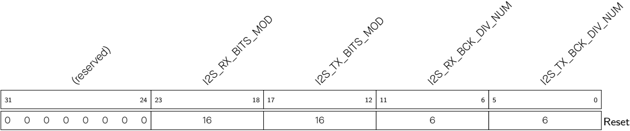
Register 12.32. I2S_SAMPLE_RATE_CONF_REG (0x00b0)
