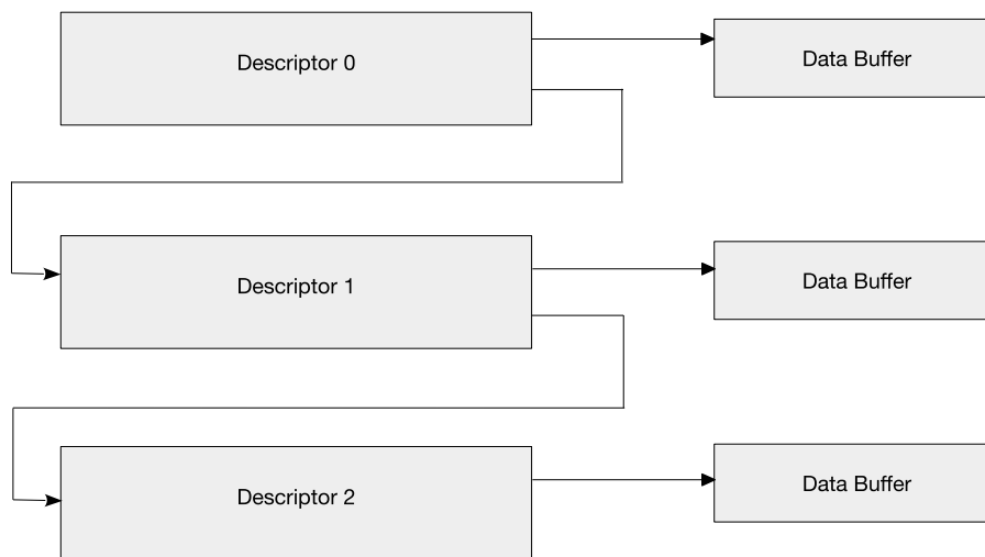
Figure 9-7. Descriptor Chain
