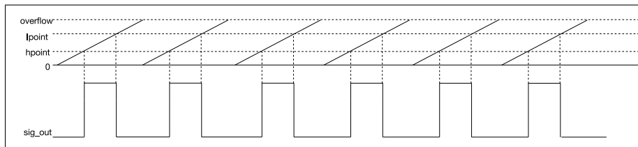
Figure 14-4. LED PWM Output Signal Diagram
