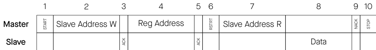
Figure 30-21. I 2 C Read Operation
