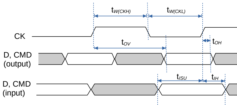
Figure 9-9. SD/MMC Timing in HS Mode
