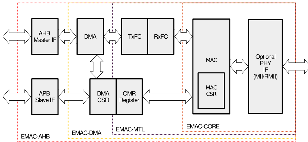
Figure 10-2. Ethernet Block Diagram
