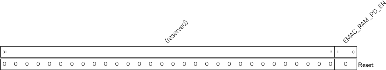
Register 10.48. EMAC_PD_SEL_REG (0x0810)
