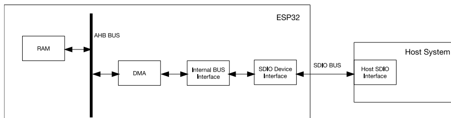
Figure 8-1. SDIO Slave Block Diagram
