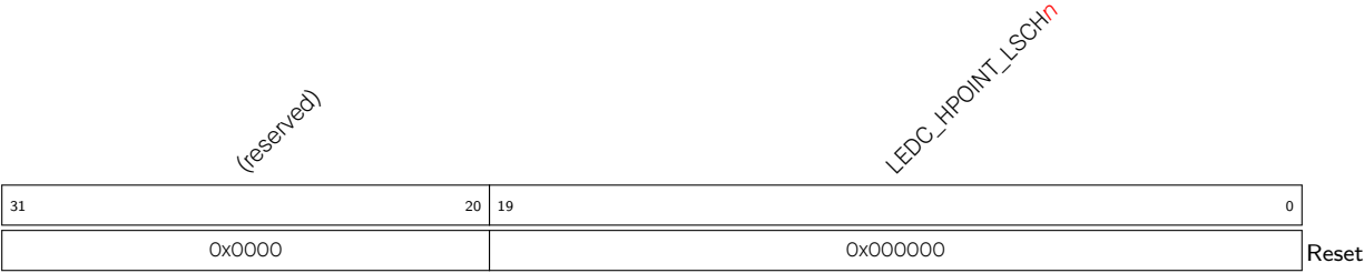
Register 14.7. LEDC_LSCH n _HPOINT_REG ( n : 0-7) (0xA4+0x14* n )
