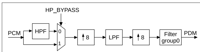
Figure 12-9. PDM Transmitting Module
