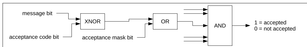
Figure 21-7. Acceptance Filter
