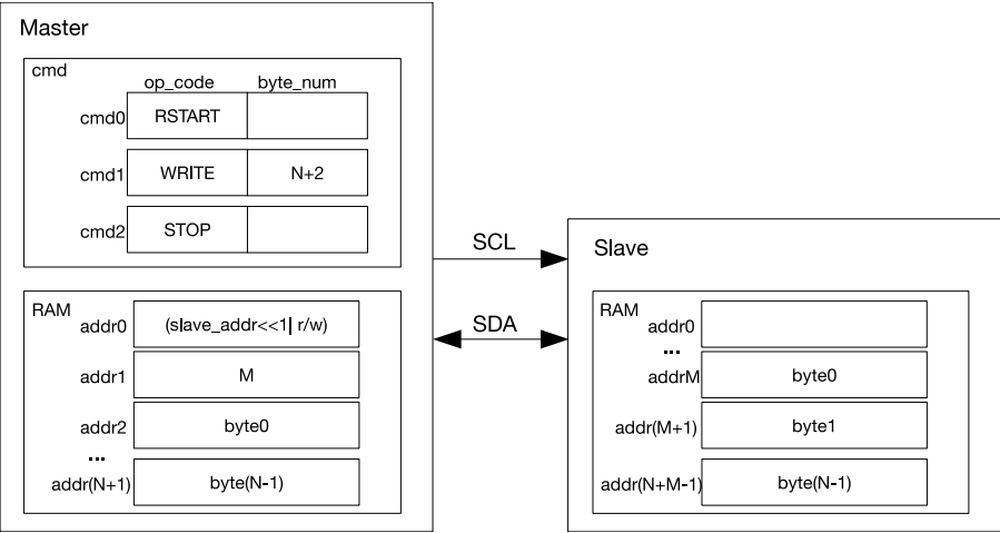
Figure 11-7. I2C Master Writes to addrM in RAM of Slave with 7-bit Address
