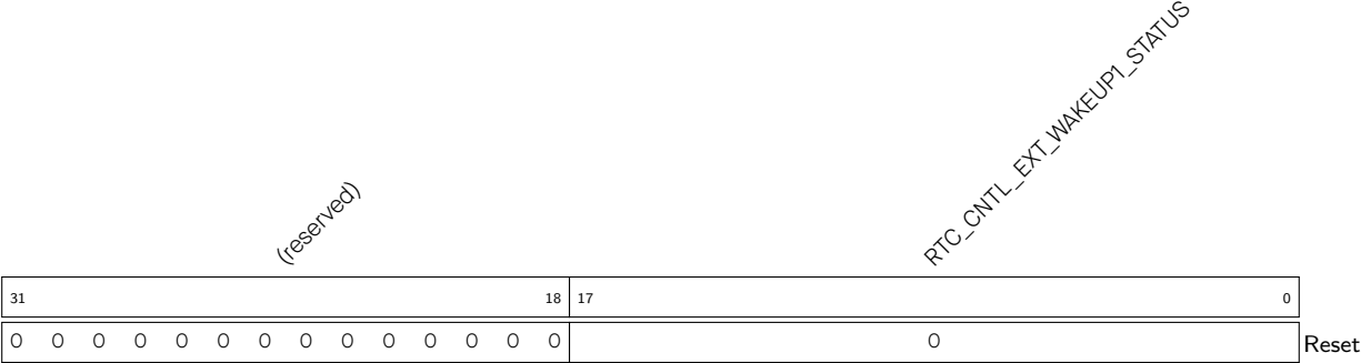
Register 31.38. RTC_CNTL_EXT_WAKEUP1_STATUS_REG (0x00D0)
