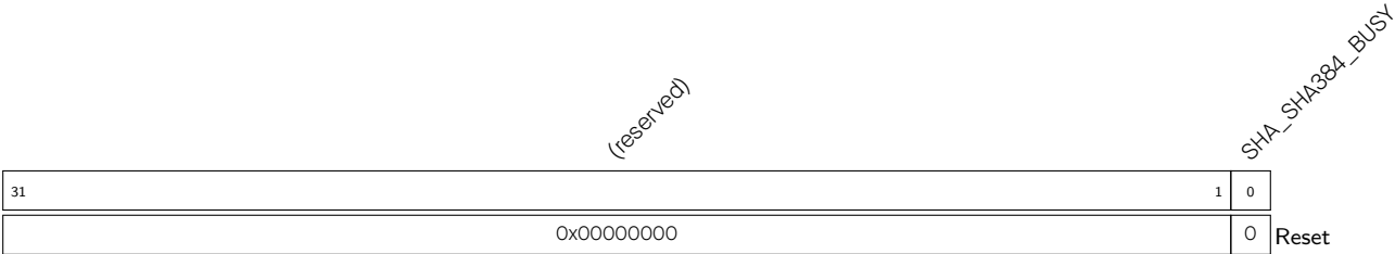
Register 23.13. SHA_SHA384_BUSY_REG (0x0AC)
