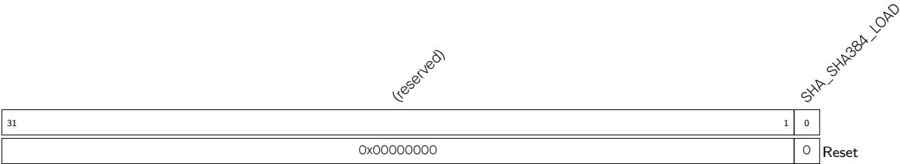
Register 23.12. SHA_SHA384_LOAD_REG (0x0A8)
