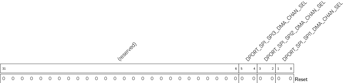
Register 5.194. DPORT_SPI_DMA_CHAN_SEL_REG (0x5A8)
