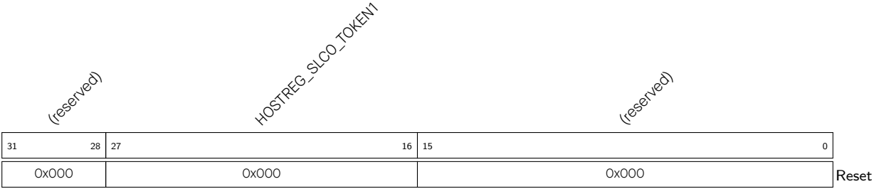
Register 8.14. SLCOHOST_TOKEN_RDATA (0x44)
