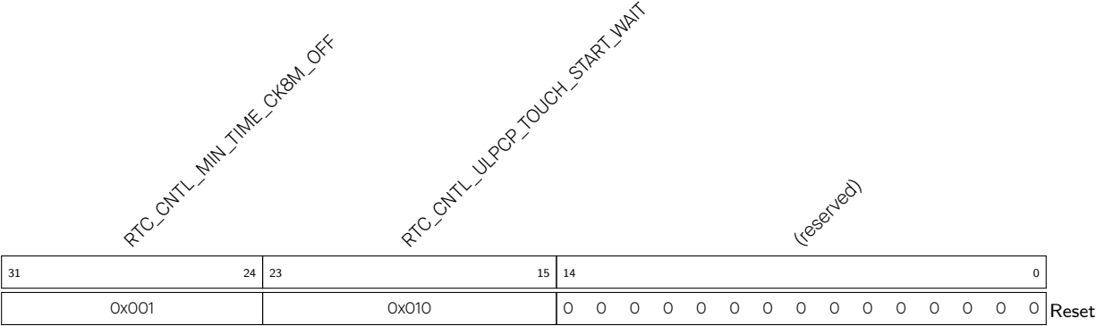
Register 31.9. RTC_CNTL_TIMER2_REG (0x0020)
