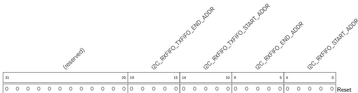
Register 11.6. I2C_RXFIFO_ST_REG (0x0014)
