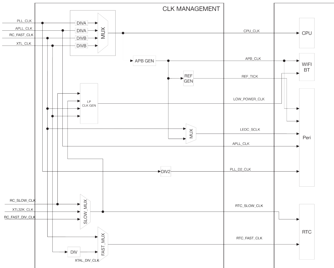
Figure 3-2. System Clock
