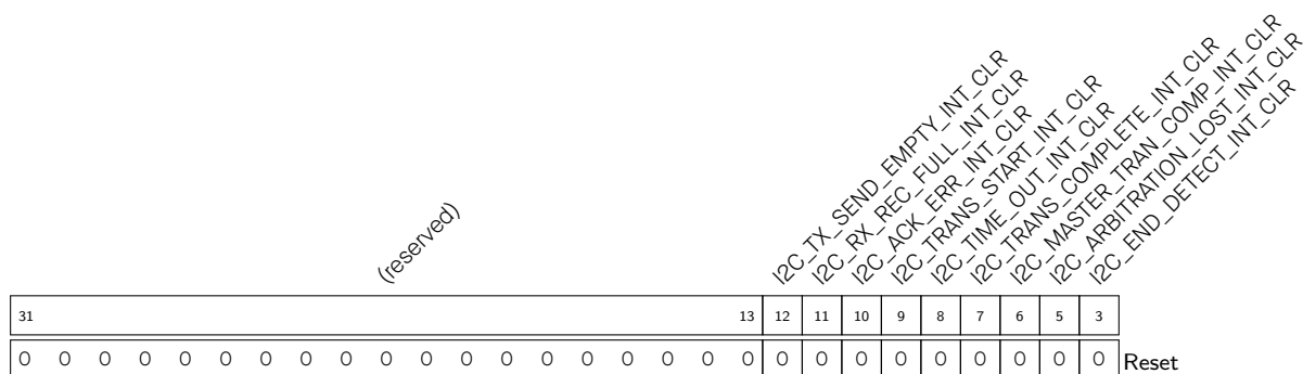
Register 11.9. I2C_INT_CLR_REG (0x0024)
