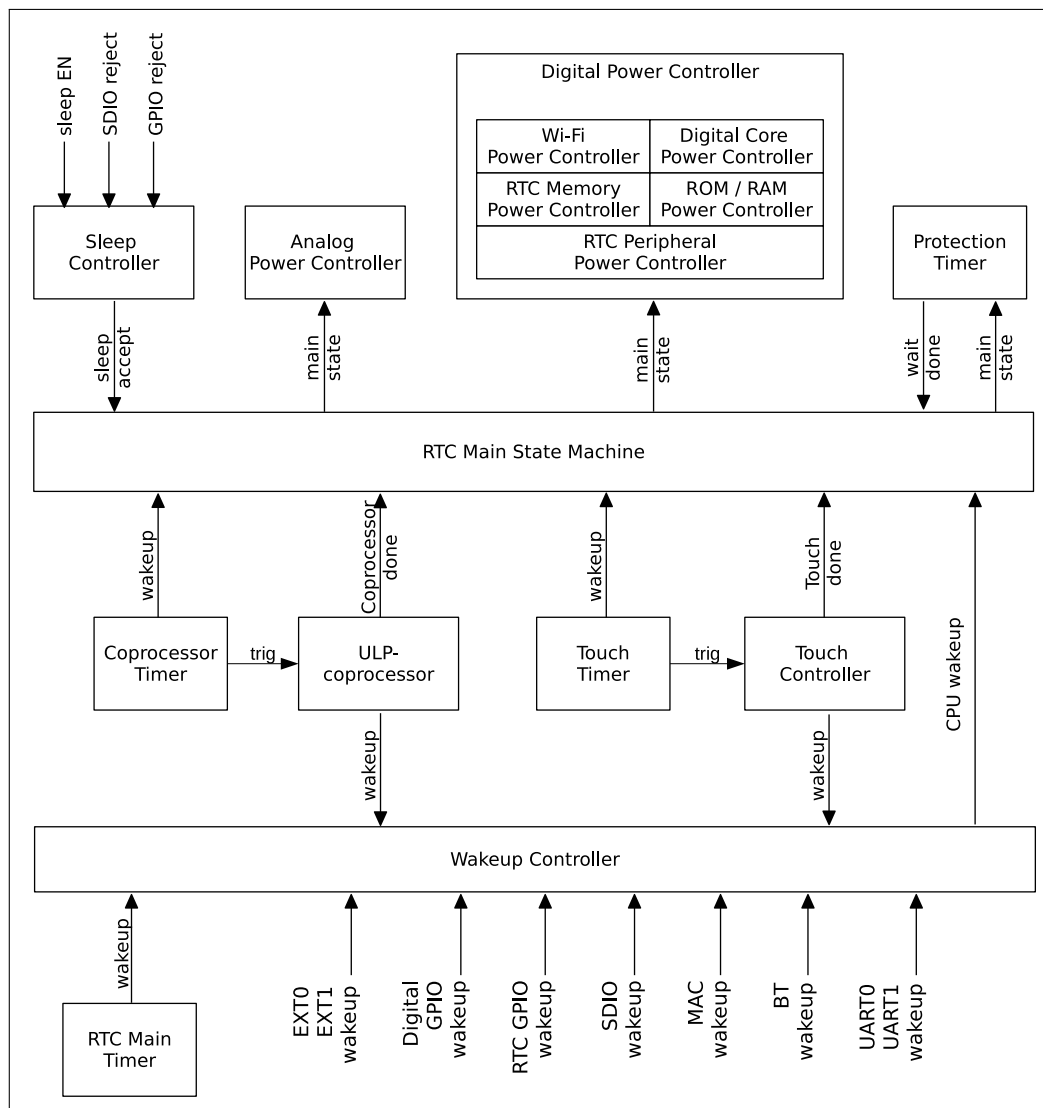
Figure 31-6. RTC Structure
