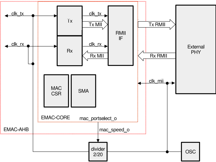
Figure 10-6. RMII Clock
