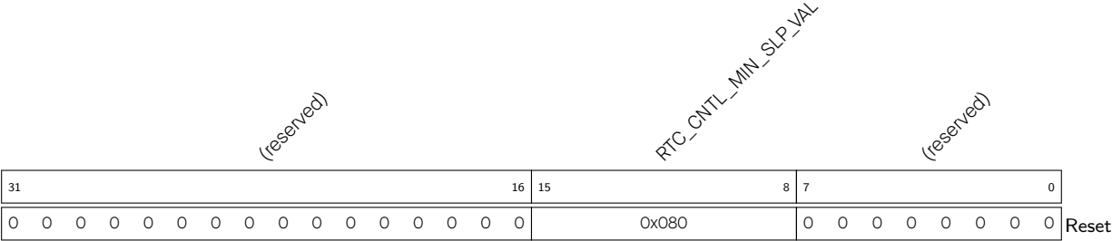
Register 31.10. RTC_CNTL_TIMER5_REG (0x002C)
