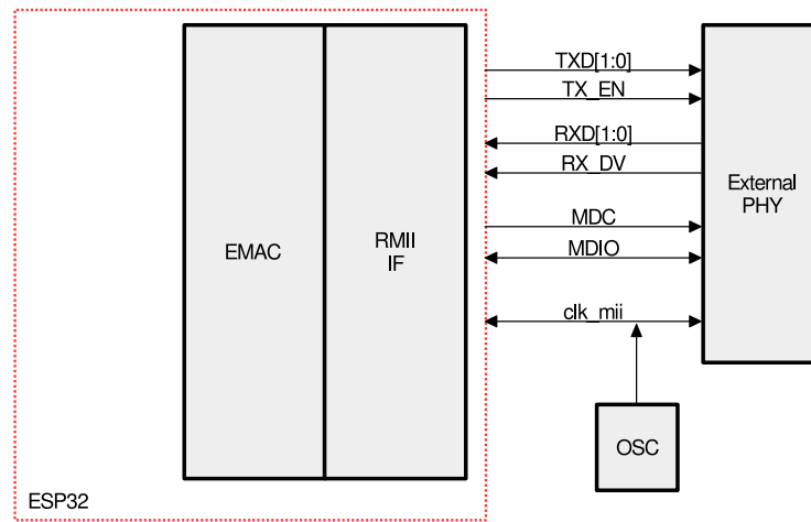
Figure 10-5. RMII Interface
