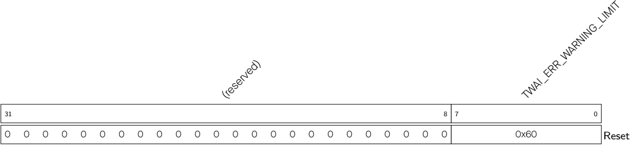
Register 21.4. TWAI_ERR_WARNING_LIMIT_REG (0x0034)
