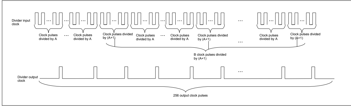
Figure 14-3. LED_PWM Divider
