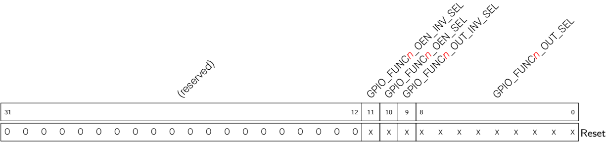
Register 4.32. GPIO_FUNCn_OUT_SEL_CFG_REG (n: 0-19, 21-23, 25-27, 32-33) (0x530+0x4*n)
