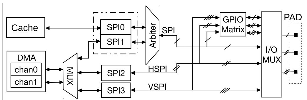
Figure 7-1. SPI Architecture
