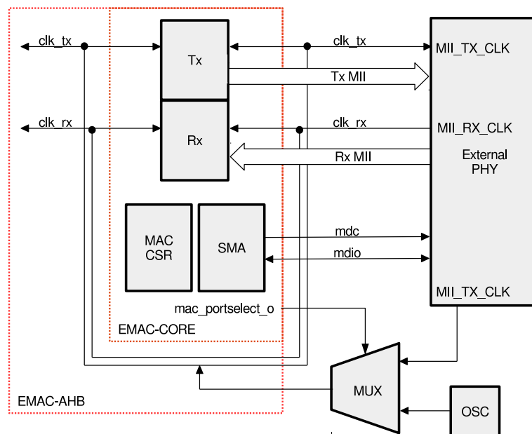
Figure 10-4. MII Clock
