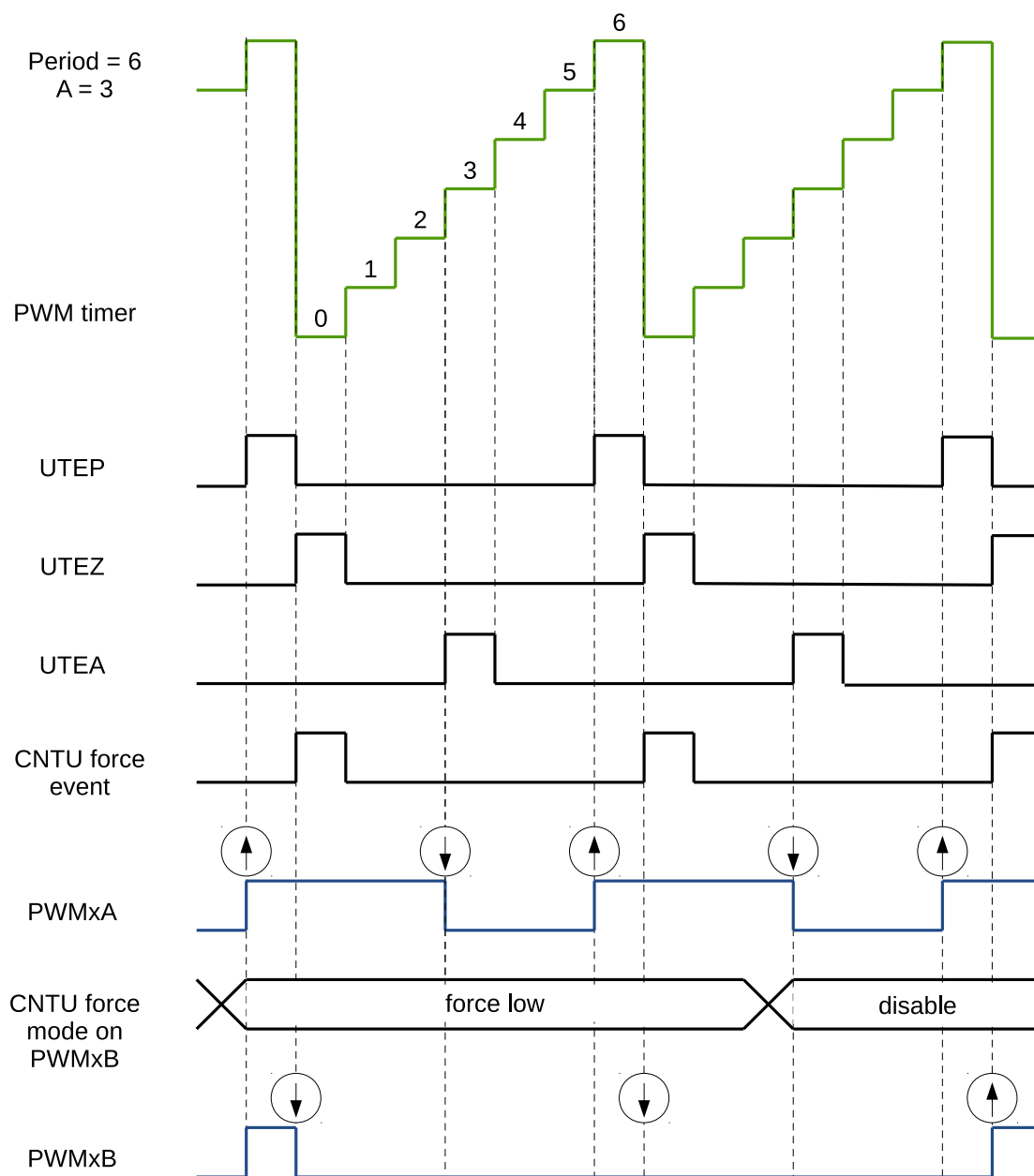
Figure 16-21. Example of a CNTU Software-Force Event on PWMxB
