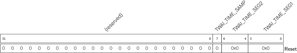
Register 21.3. TWAI_BUS_TIMING_1_REG (0x001C)
