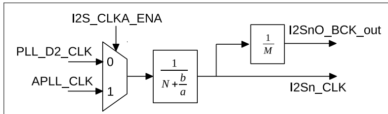
Figure 12-2. I2S Clock
