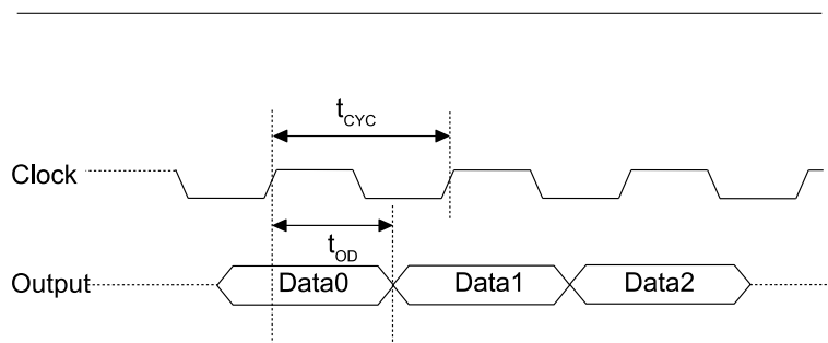
Figure 10-8. RMII Timing – Transmitting Data
