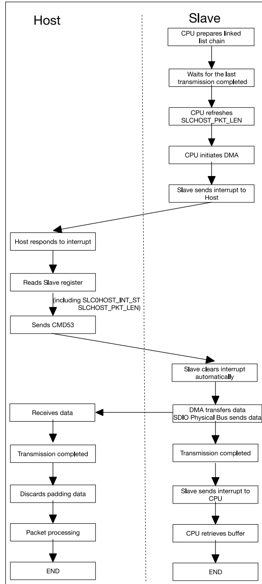
Figure 8-6. Packet Sending Procedure (Initiated by Slave)
