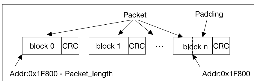
Figure 8-2. SDIO Bus Packet Transmission
