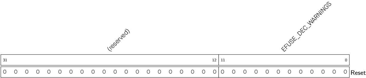
Register 20.29. EFUSE_DEC_STATUS_REG (0x11c)
