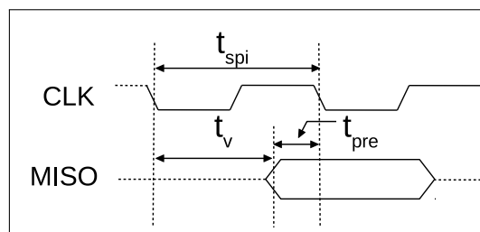
Figure 7-4. GP-SPI Slave Data Output
