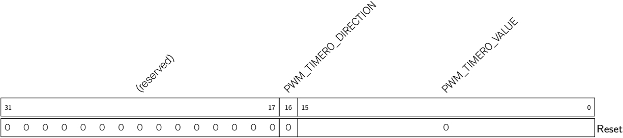
Register 16.5. PWM_TIMER0_STATUS_REG (0x0010)
