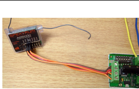
Figure 5.1: R/C connection
