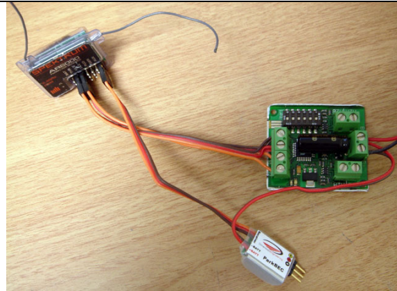
Figure 5.2: R/C with a ParkBEC
