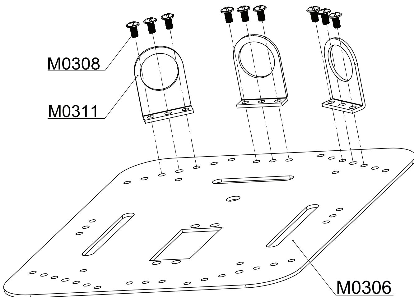
A1 M0311x3 红外传感器支架 IR Sensor Mounting Bracket
