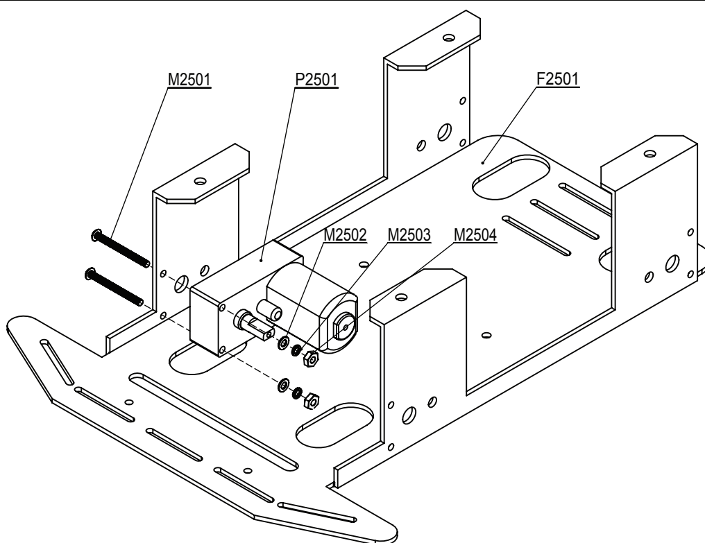
A1 M2501x2 M2.5x25mm 半圆头十字螺丝 Philips Truss Screw (M2.5X25mm)
