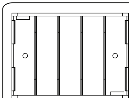
A1 P2502x1 电池盒 Battery Holder
