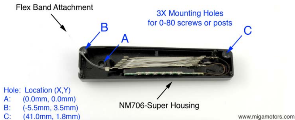
Mounting Options for NM706-Super
