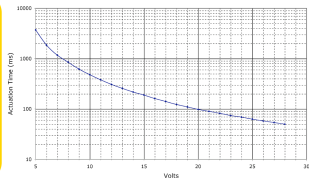
MigaOne™ Actuation Time
