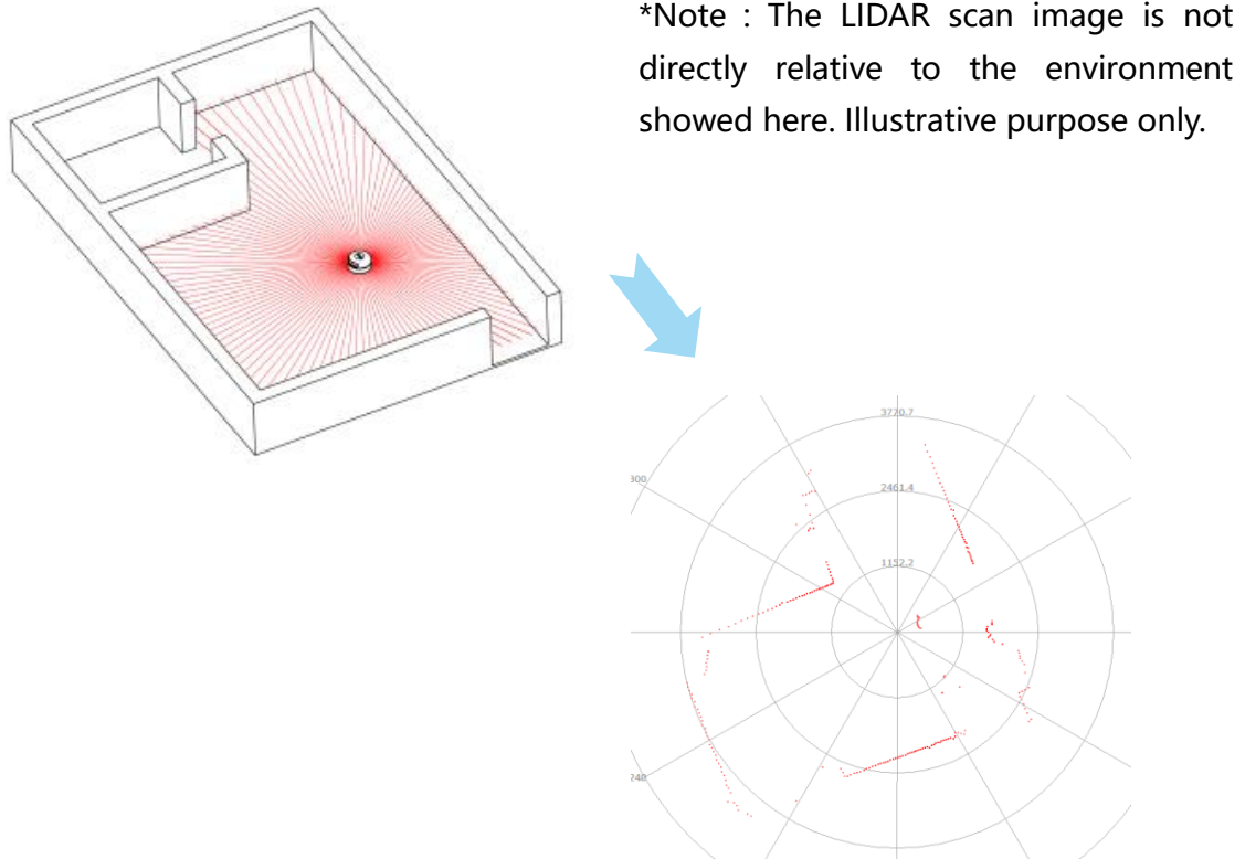
Figure 1-3 The Obtained Environment Map from RPLIDAR Scanning
