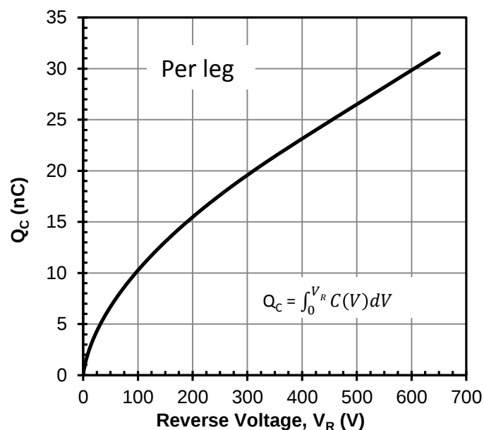
Figure 8 Typical capacitive charge per leg vs. reverse voltage
