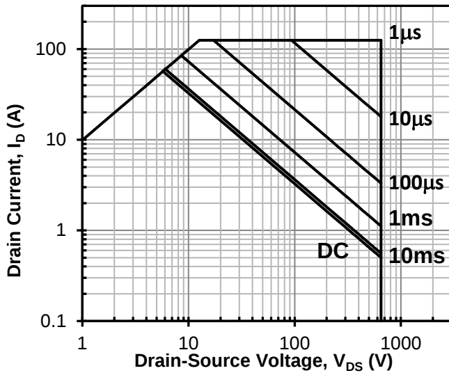
Figure 17 Safe operation area
